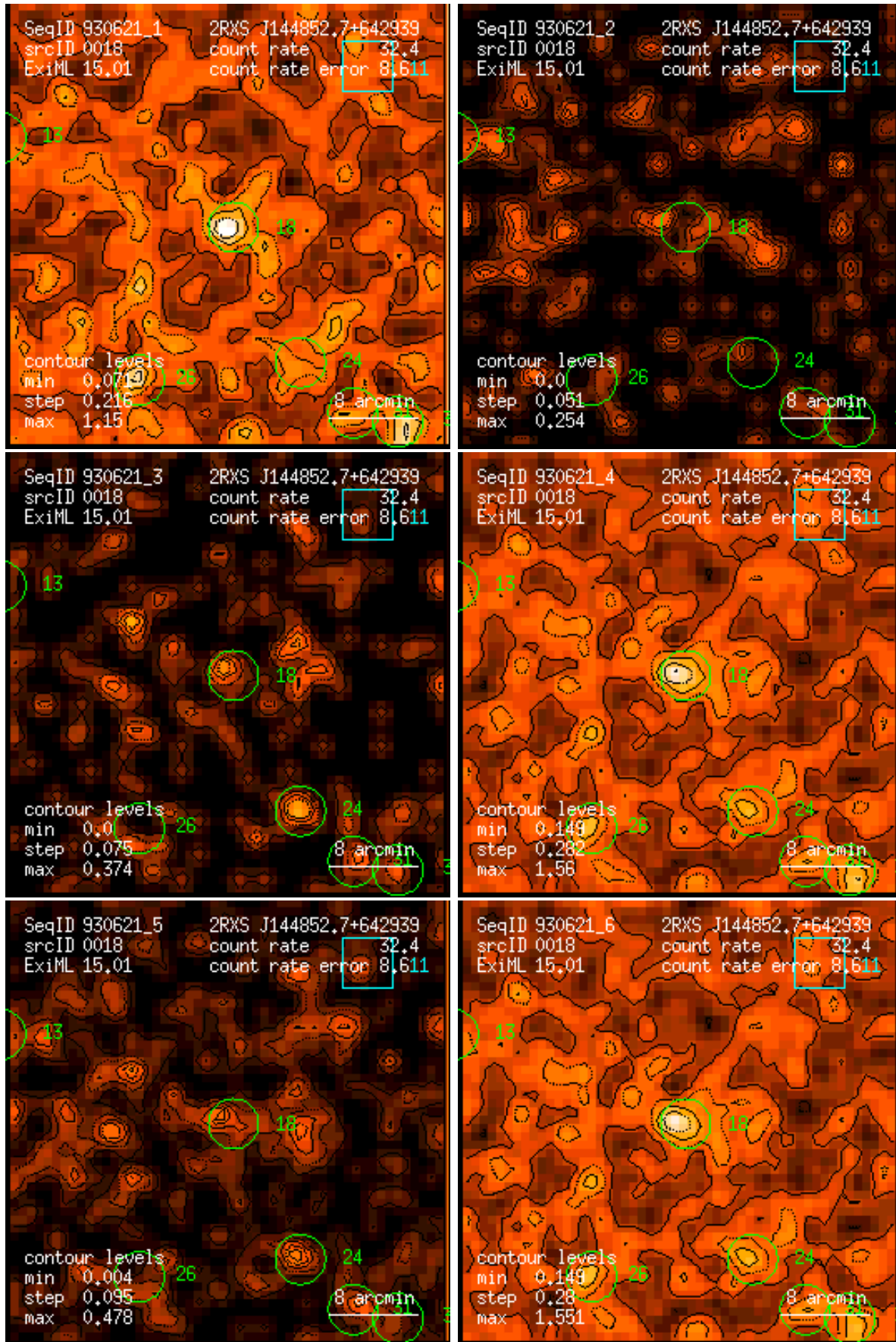
Figure 18: RASS 930621: detection 0018: band rate images, Gaussian filter: (1) PSPC channels 11 – 41, (2) 52 – 90, (3) 91 – 201, (4) 11 – 235, (5) 52 – 201, (6) 11 – 201. Broad band rates in counts/ks. Band rate contour levels in counts/ks/arcmin 2 .
