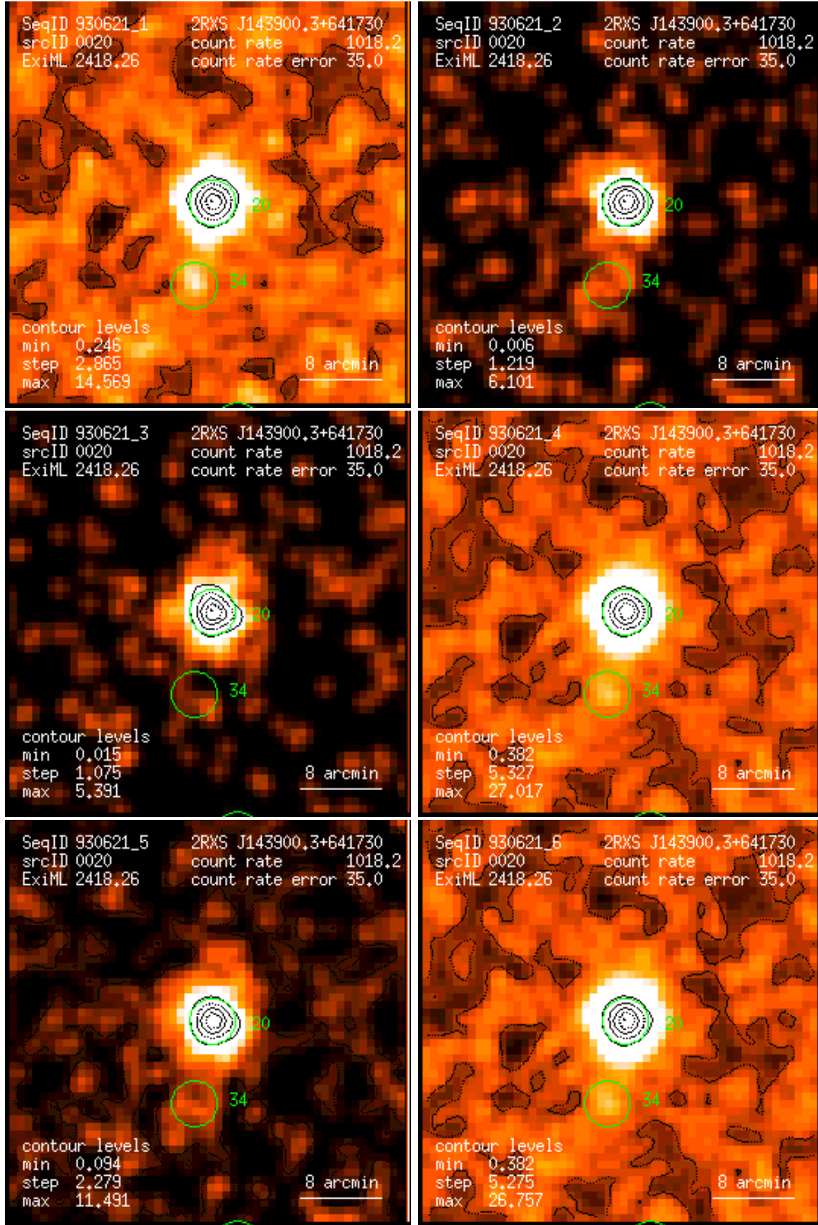
Figure 20: RASS 930621: detection 0020: band rate images, Gaussian filter: (1) PSPC channels 11 – 41, (2) 52 – 90, (3) 91 – 201, (4) 11 – 235, (5) 52 – 201, (6) 11 – 201. Broad band rates in counts/ks. Band rate contour levels in counts/ks/arcmin 2 .
