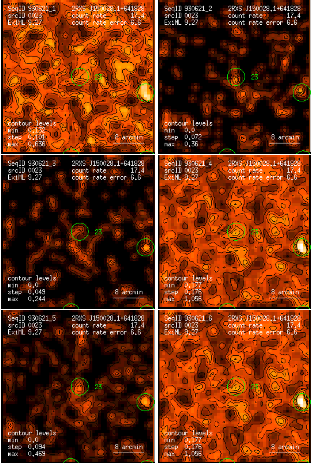
Figure 23: RASS 930621: detection 0023: band rate images, Gaussian filter: (1) PSPC channels 11 – 41, (2) 52 – 90, (3) 91 – 201, (4) 11 – 235, (5) 52 – 201, (6) 11 – 201. Broad band rates in counts/ks. Band rate contour levels in counts/ks/arcmin 2 .
