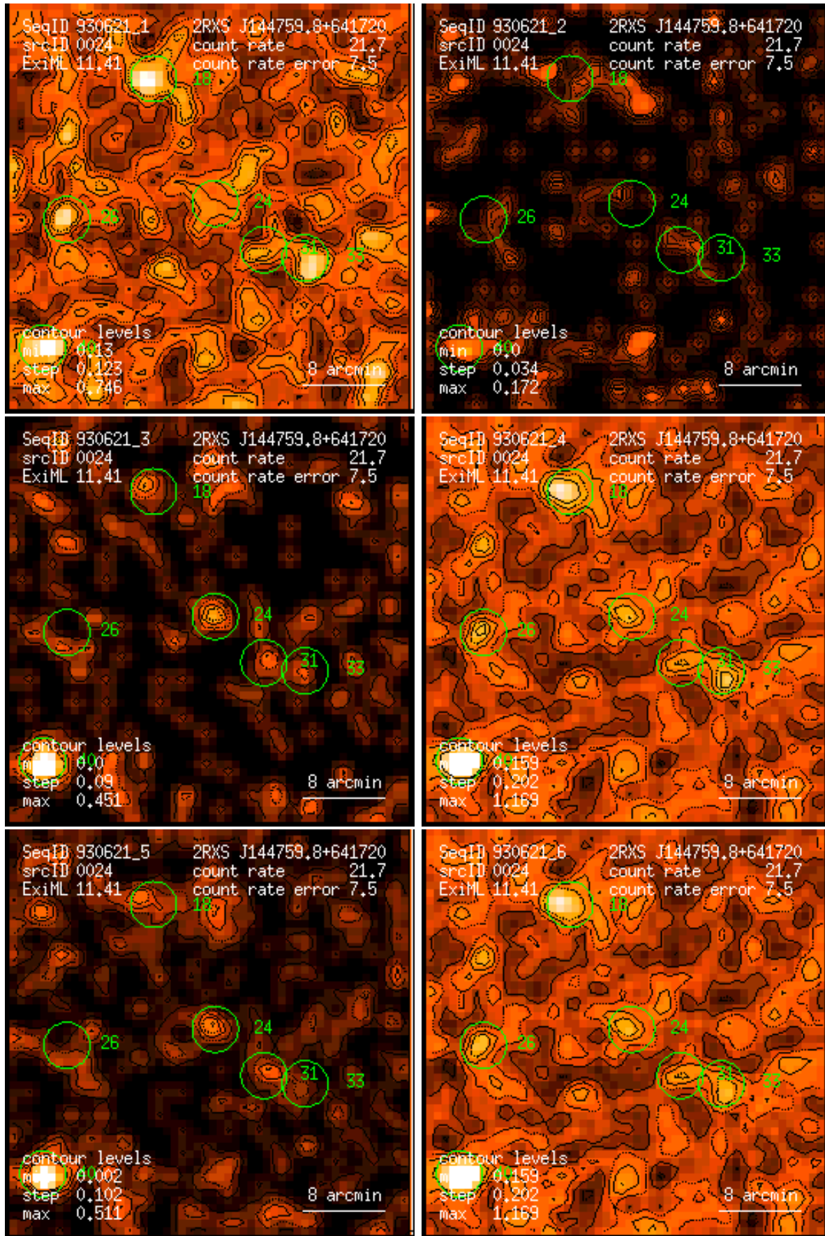
Figure 24: RASS 930621: detection 0024: band rate images, Gaussian filter: (1) PSPC channels 11 – 41, (2) 52 – 90, (3) 91 – 201, (4) 11 – 235, (5) 52 – 201, (6) 11 – 201. Broad band rates in counts/ks. Band rate contour levels in counts/ks/arcmin 2 .
