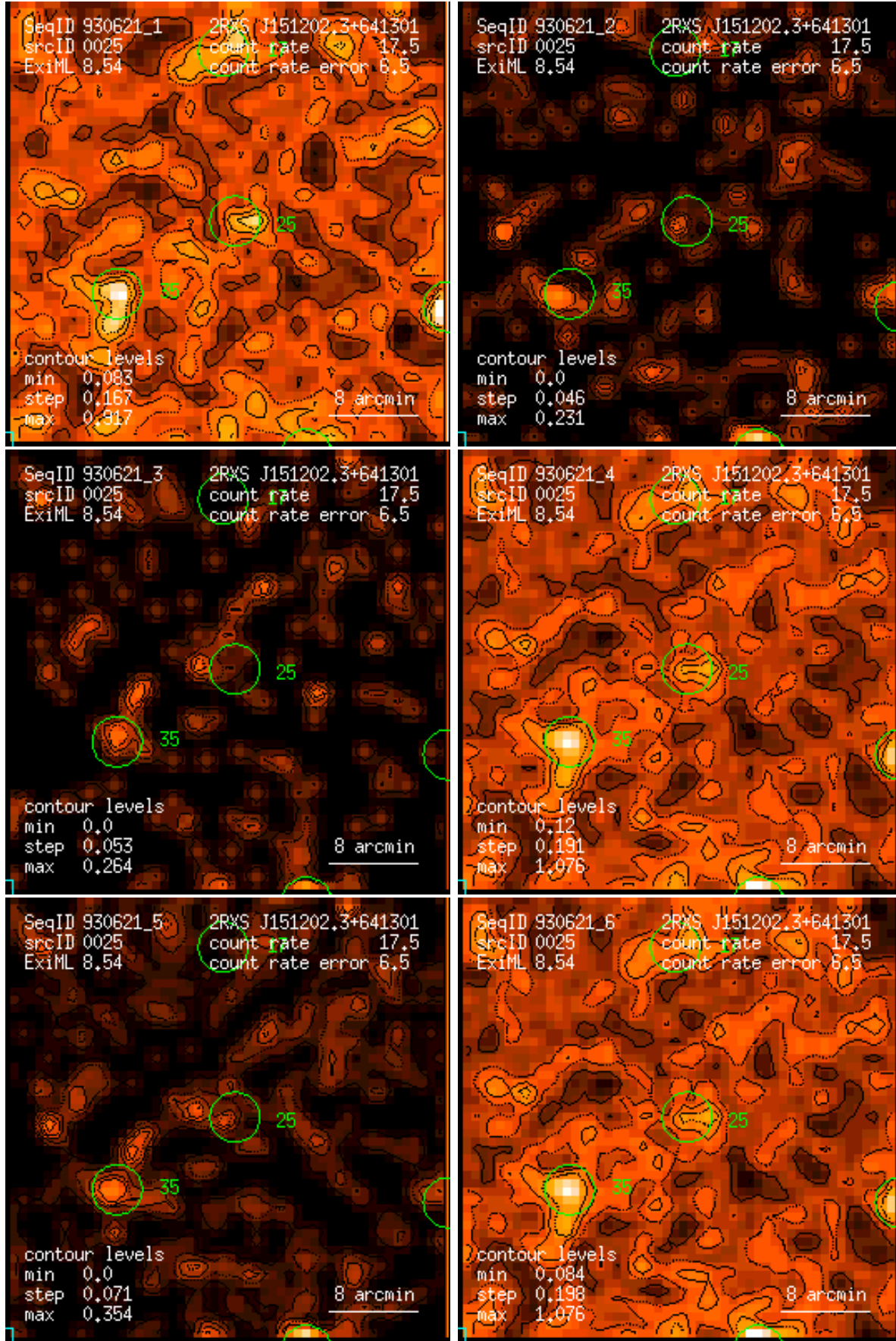
Figure 25: RASS 930621: detection 0025: band rate images, Gaussian filter: (1) PSPC channels 11 – 41, (2) 52 – 90, (3) 91 – 201, (4) 11 – 235, (5) 52 – 201, (6) 11 – 201. Broad band rates in counts/ks. Band rate contour levels in counts/ks/arcmin 2 .
