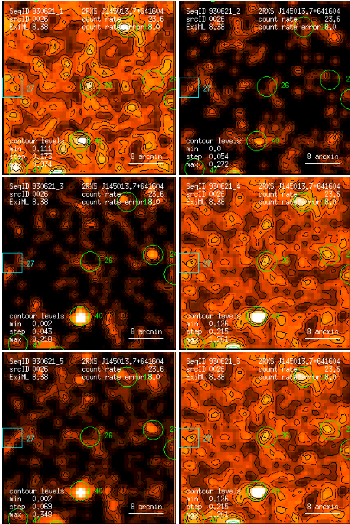
Figure 26: RASS 930621: detection 0026: band rate images, Gaussian filter: (1) PSPC channels 11 – 41, (2) 52 – 90, (3) 91 – 201, (4) 11 – 235, (5) 52 – 201, (6) 11 – 201. Broad band rates in counts/ks. Band rate contour levels in counts/ks/arcmin 2 .
