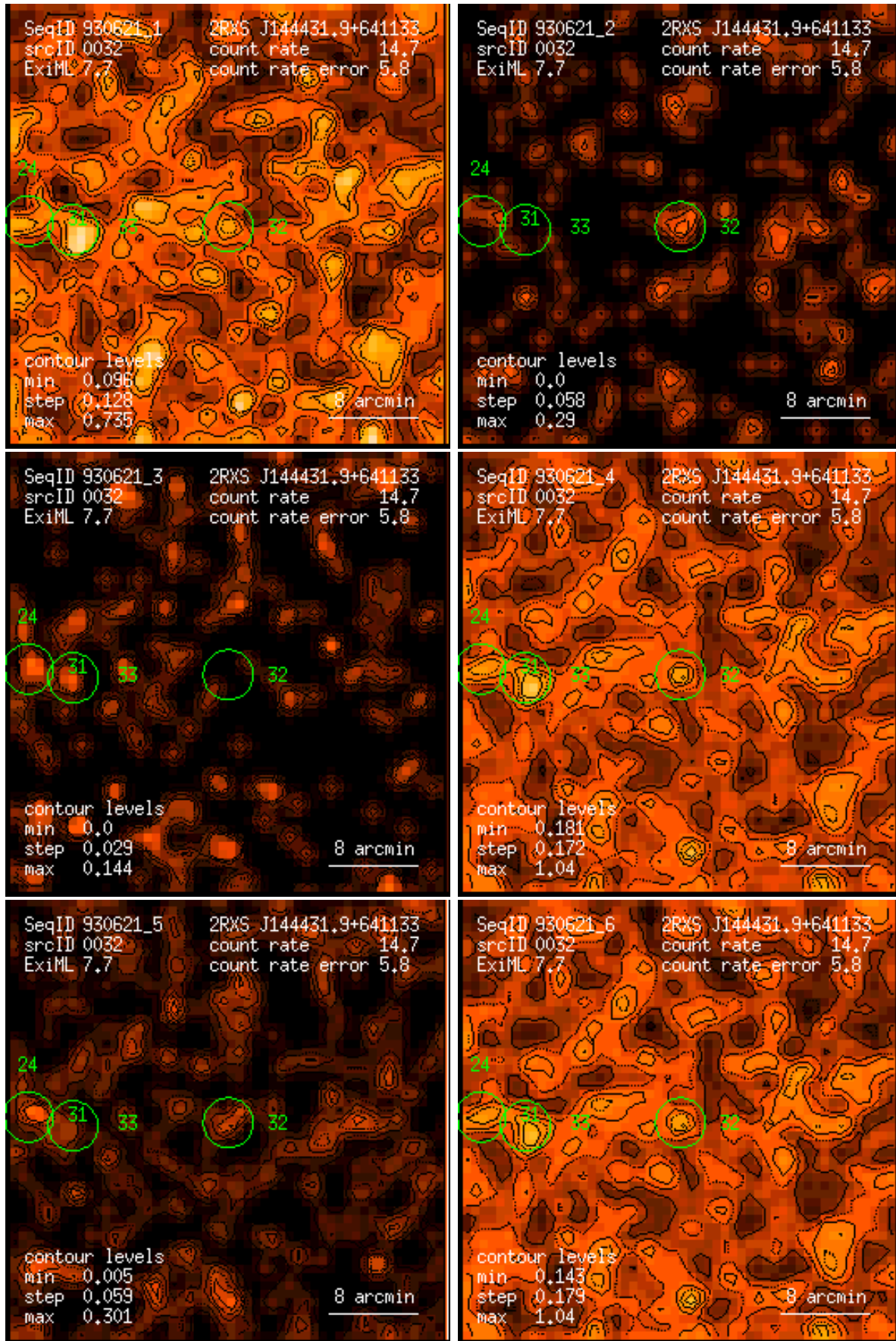
Figure 32: RASS 930621: detection 0032: band rate images, Gaussian filter: (1) PSPC channels 11 – 41, (2) 52 – 90, (3) 91 – 201, (4) 11 – 235, (5) 52 – 201, (6) 11 – 201. Broad band rates in counts/ks. Band rate contour levels in counts/ks/arcmin 2 .
