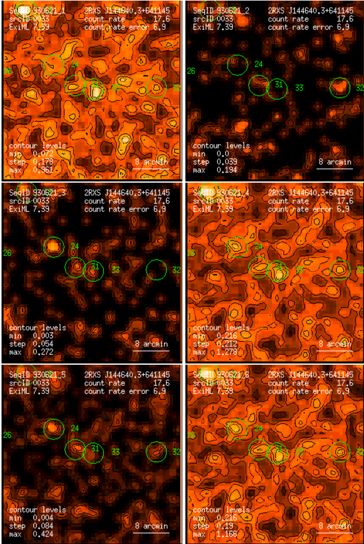
Figure 33: RASS 930621: detection 0033: band rate images, Gaussian filter: (1) PSPC channels 11 – 41, (2) 52 – 90, (3) 91 – 201, (4) 11 – 235, (5) 52 – 201, (6) 11 – 201. Broad band rates in counts/ks. Band rate contour levels in counts/ks/arcmin 2 .
