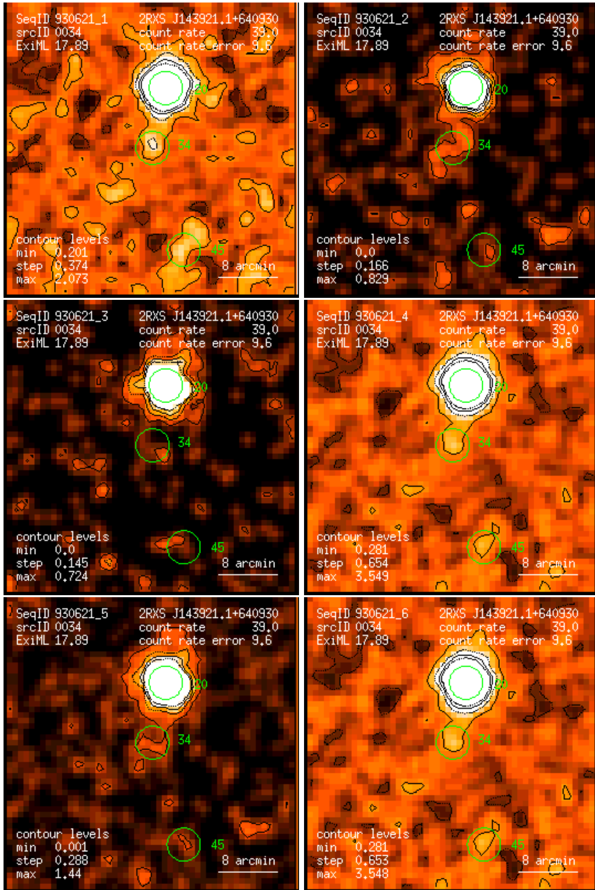
Figure 34: RASS 930621: detection 0034: band rate images, Gaussian filter: (1) PSPC channels 11 – 41, (2) 52 – 90, (3) 91 – 201, (4) 11 – 235, (5) 52 – 201, (6) 11 – 201. Broad band rates in counts/ks. Band rate contour levels in counts/ks/arcmin 2 .
