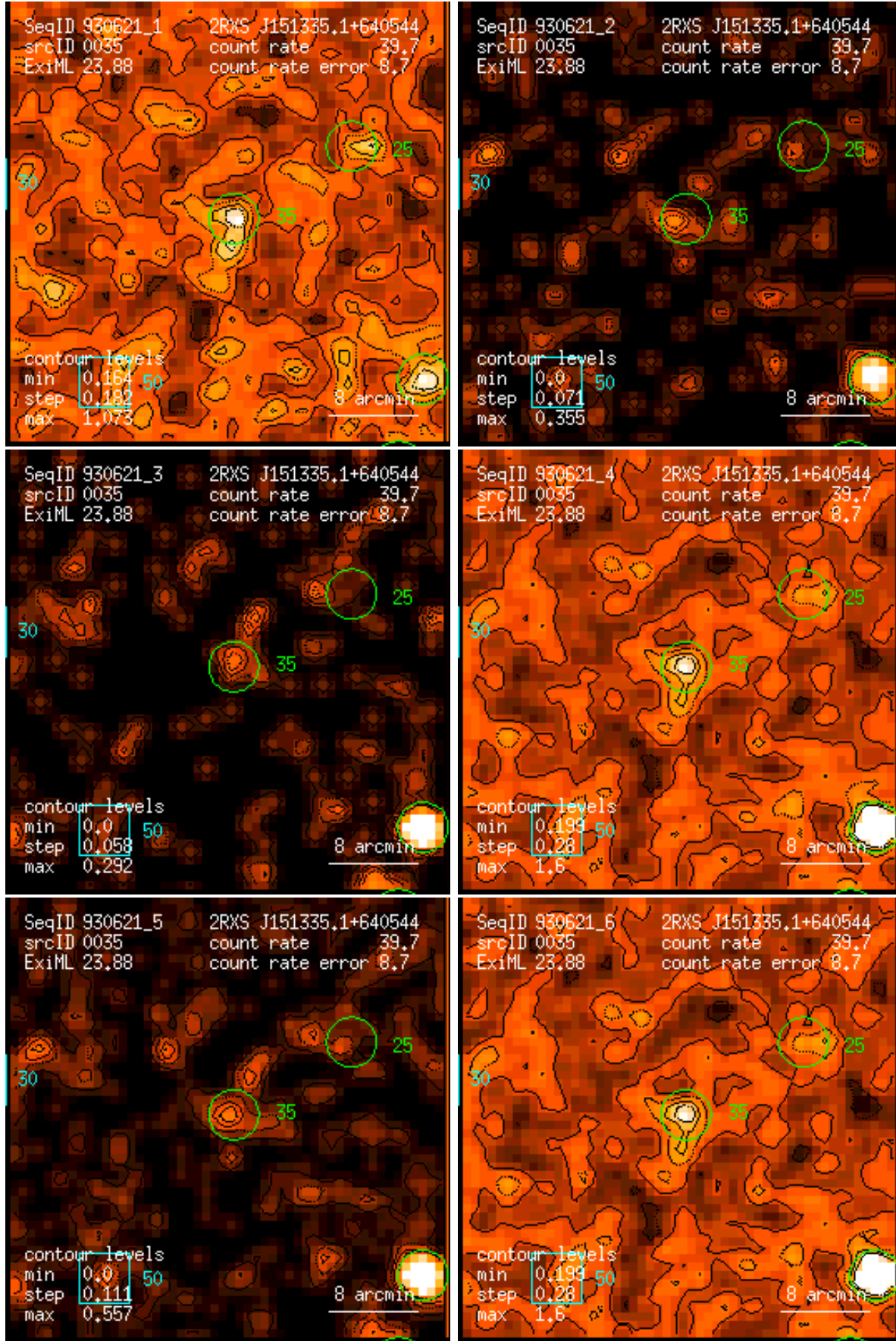
Figure 35: RASS 930621: detection 0035: band rate images, Gaussian filter: (1) PSPC channels 11 – 41, (2) 52 – 90, (3) 91 – 201, (4) 11 – 235, (5) 52 – 201, (6) 11 – 201. Broad band rates in counts/ks. Band rate contour levels in counts/ks/arcmin 2 .
