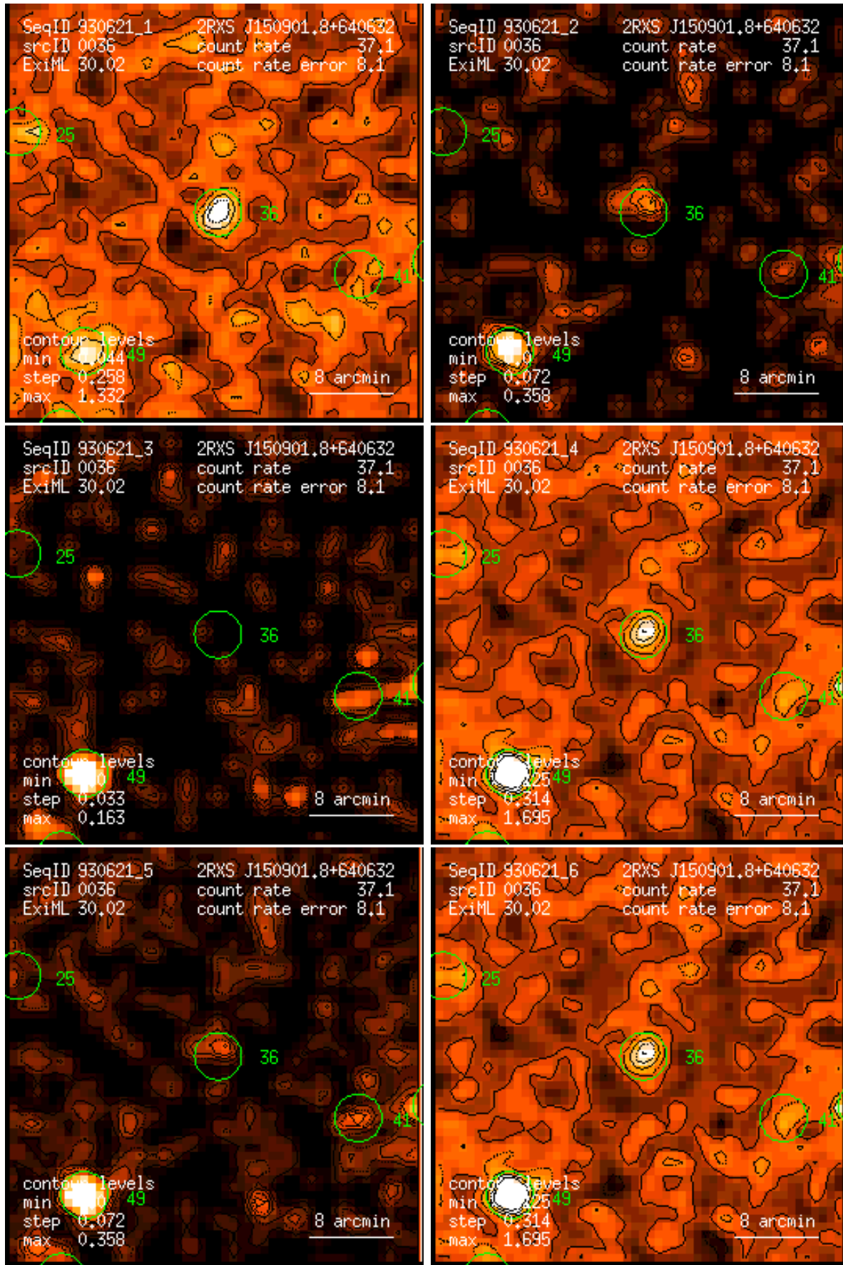
Figure 36: RASS 930621: detection 0036: band rate images, Gaussian filter: (1) PSPC channels 11 – 41, (2) 52 – 90, (3) 91 – 201, (4) 11 – 235, (5) 52 – 201, (6) 11 – 201. Broad band rates in counts/ks. Band rate contour levels in counts/ks/arcmin 2 .
