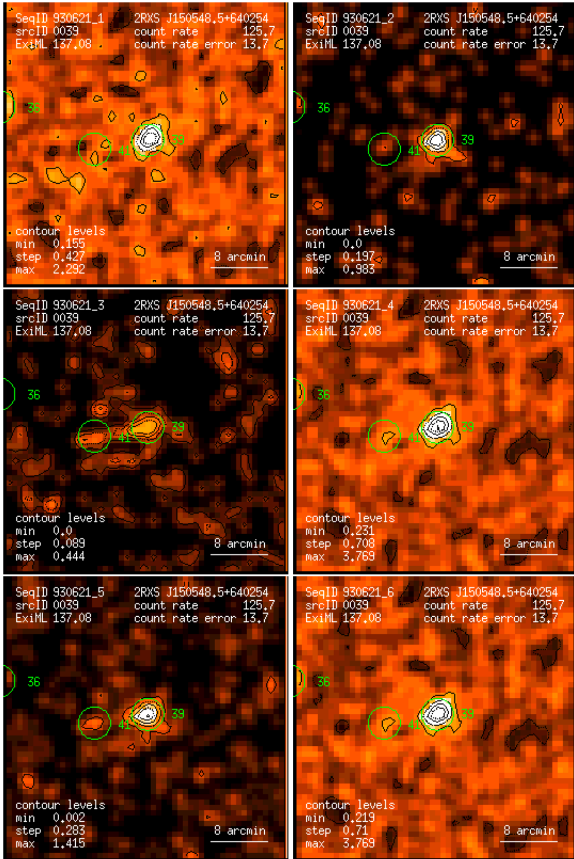
Figure 39: RASS 930621: detection 0039: band rate images, Gaussian filter: (1) PSPC channels 11 – 41, (2) 52 – 90, (3) 91 – 201, (4) 11 – 235, (5) 52 – 201, (6) 11 – 201. Broad band rates in counts/ks. Band rate contour levels in counts/ks/arcmin 2 .
