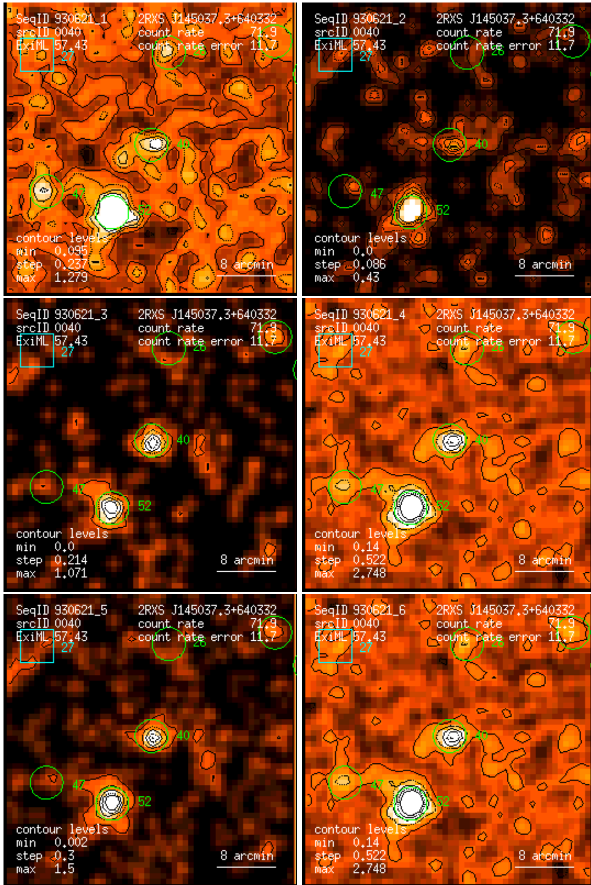
Figure 40: RASS 930621: detection 0040: band rate images, Gaussian filter: (1) PSPC channels 11 – 41, (2) 52 – 90, (3) 91 – 201, (4) 11 – 235, (5) 52 – 201, (6) 11 – 201. Broad band rates in counts/ks. Band rate contour levels in counts/ks/arcmin 2 .
