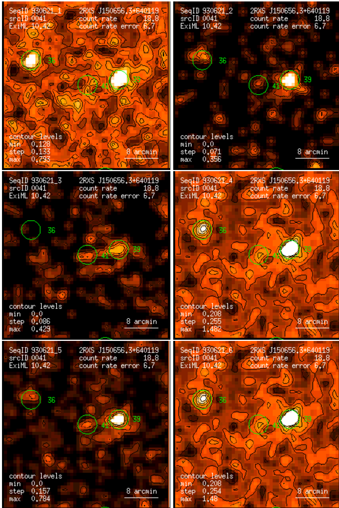
Figure 41: RASS 930621: detection 0041: band rate images, Gaussian filter: (1) PSPC channels 11 – 41, (2) 52 – 90, (3) 91 – 201, (4) 11 – 235, (5) 52 – 201, (6) 11 – 201. Broad band rates in counts/ks. Band rate contour levels in counts/ks/arcmin 2 .
