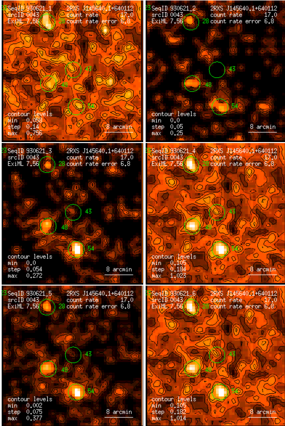
Figure 43: RASS 930621: detection 0043: band rate images, Gaussian filter: (1) PSPC channels 11 – 41, (2) 52 – 90, (3) 91 – 201, (4) 11 – 235, (5) 52 – 201, (6) 11 – 201. Broad band rates in counts/ks. Band rate contour levels in counts/ks/arcmin 2 .
