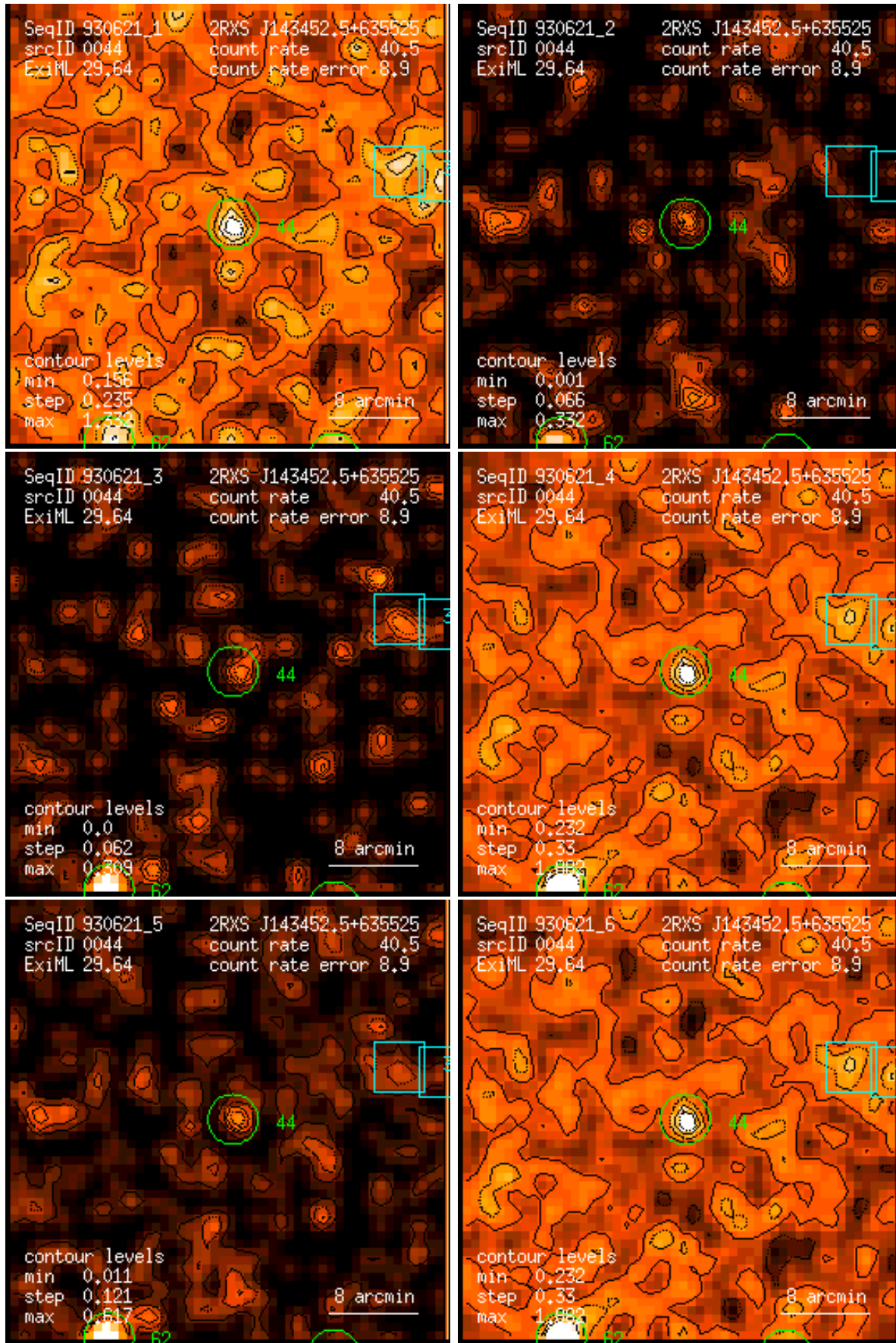
Figure 44: RASS 930621: detection 0044: band rate images, Gaussian filter: (1) PSPC channels 11 – 41, (2) 52 – 90, (3) 91 – 201, (4) 11 – 235, (5) 52 – 201, (6) 11 – 201. Broad band rates in counts/ks. Band rate contour levels in counts/ks/arcmin 2 .
