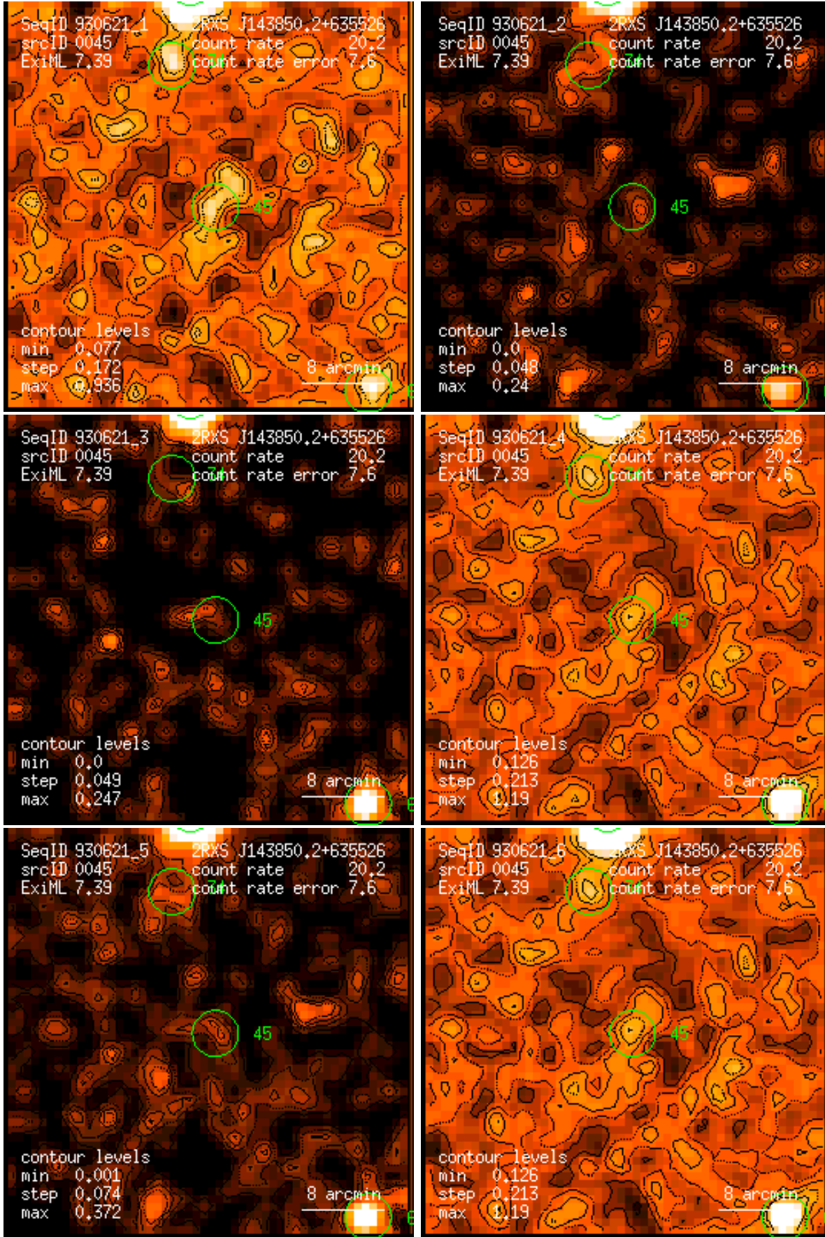
Figure 45: RASS 930621: detection 0045: band rate images, Gaussian filter: (1) PSPC channels 11 – 41, (2) 52 – 90, (3) 91 – 201, (4) 11 – 235, (5) 52 – 201, (6) 11 – 201. Broad band rates in counts/ks. Band rate contour levels in counts/ks/arcmin 2 .
