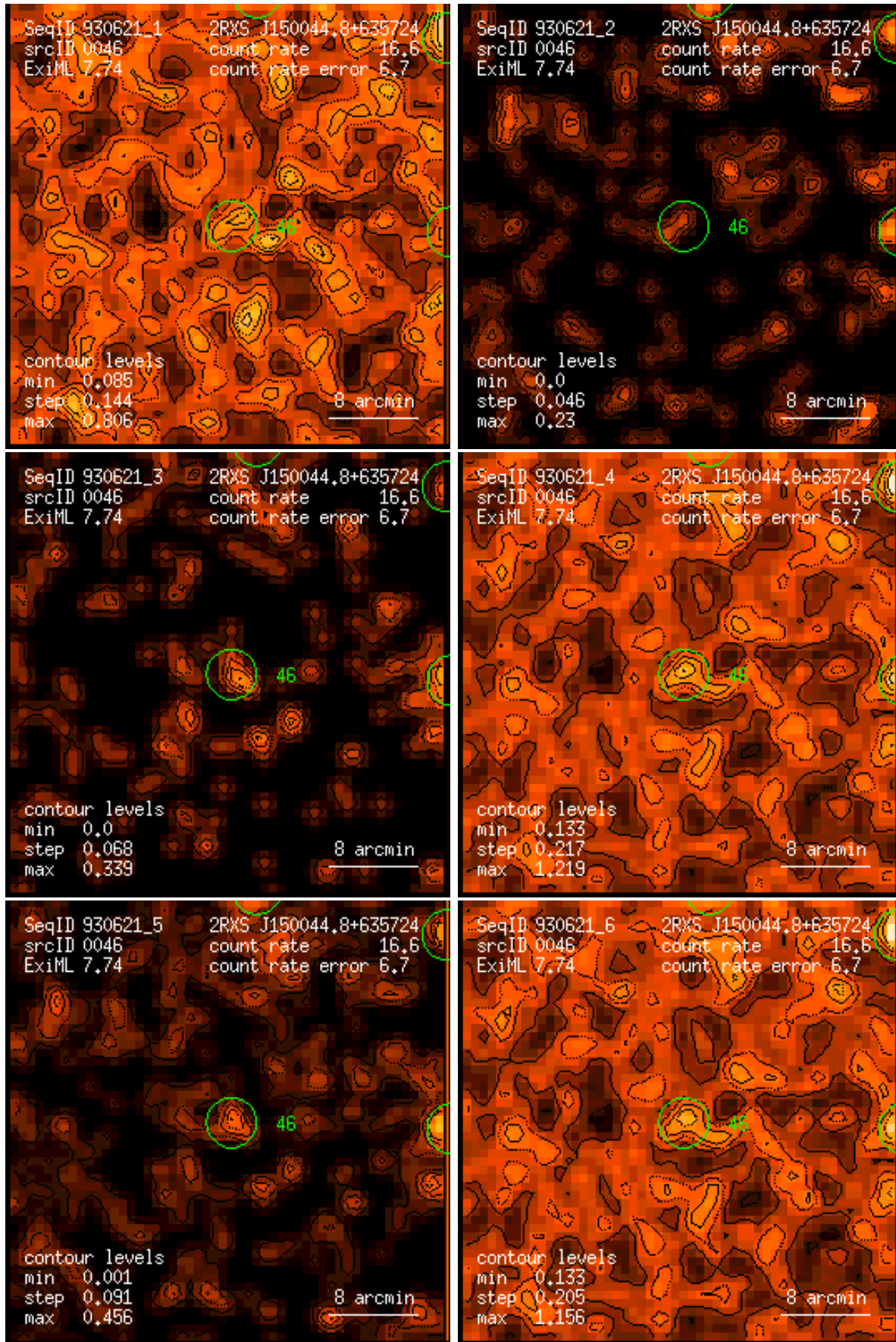
Figure 46: RASS 930621: detection 0046: band rate images, Gaussian filter: (1) PSPC channels 11 – 41, (2) 52 – 90, (3) 91 – 201, (4) 11 – 235, (5) 52 – 201, (6) 11 – 201. Broad band rates in counts/ks. Band rate contour levels in counts/ks/arcmin 2 .
