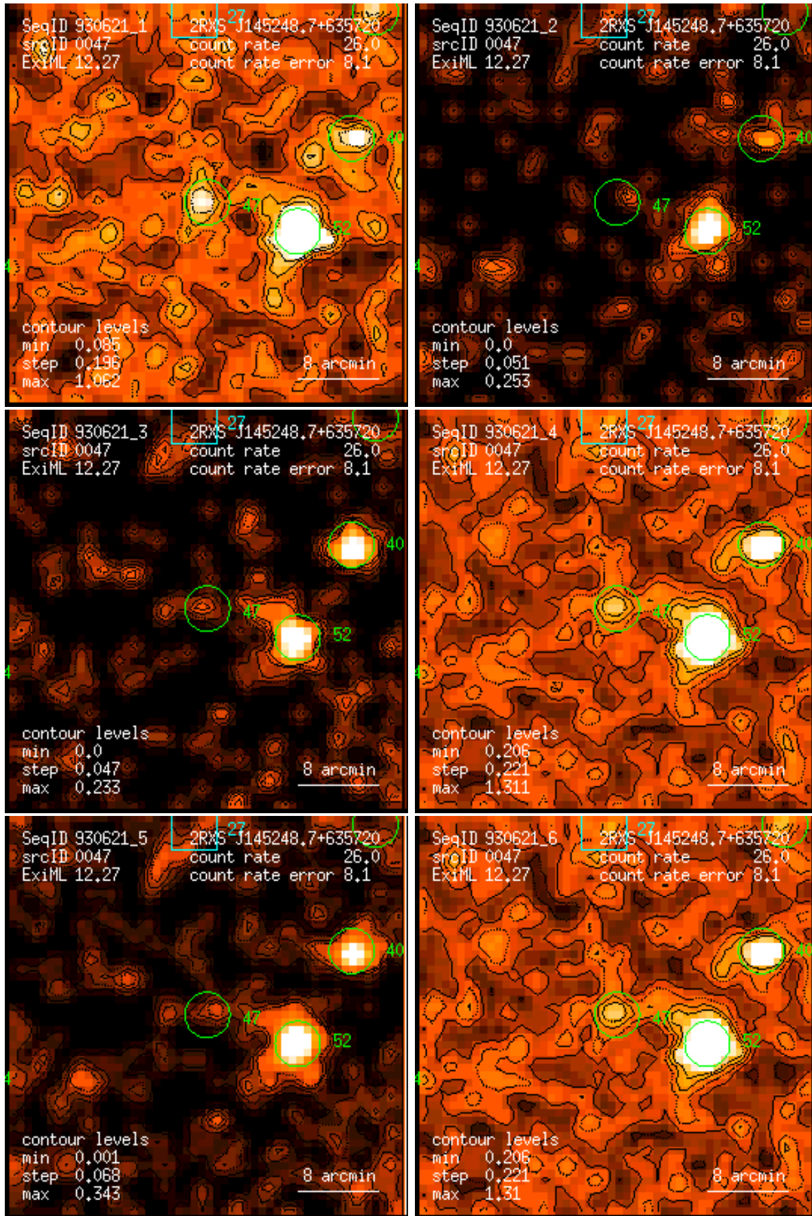
Figure 47: RASS 930621: detection 0047: band rate images, Gaussian filter: (1) PSPC channels 11 – 41, (2) 52 – 90, (3) 91 – 201, (4) 11 – 235, (5) 52 – 201, (6) 11 – 201. Broad band rates in counts/ks. Band rate contour levels in counts/ks/arcmin 2 .
