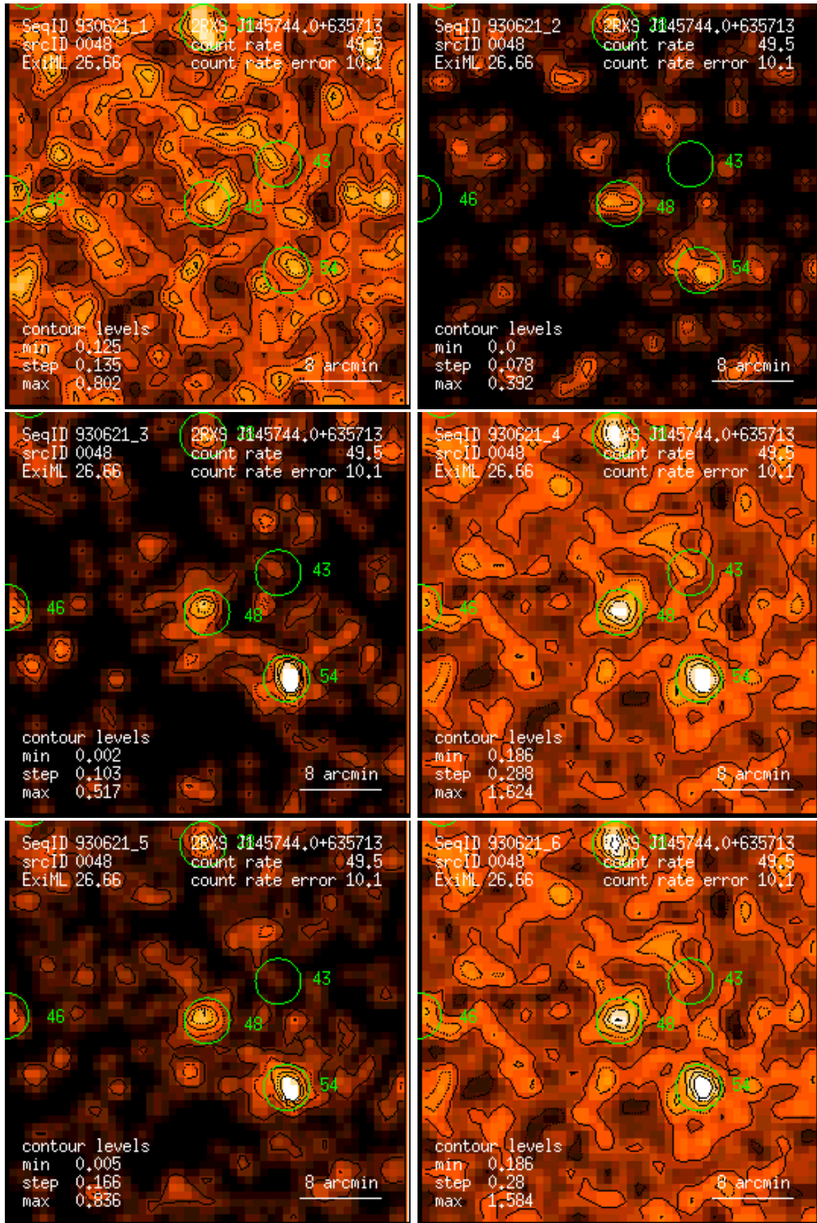
Figure 48: RASS 930621: detection 0048: band rate images, Gaussian filter: (1) PSPC channels 11 – 41, (2) 52 – 90, (3) 91 – 201, (4) 11 – 235, (5) 52 – 201, (6) 11 – 201. Broad band rates in counts/ks. Band rate contour levels in counts/ks/arcmin 2 .
