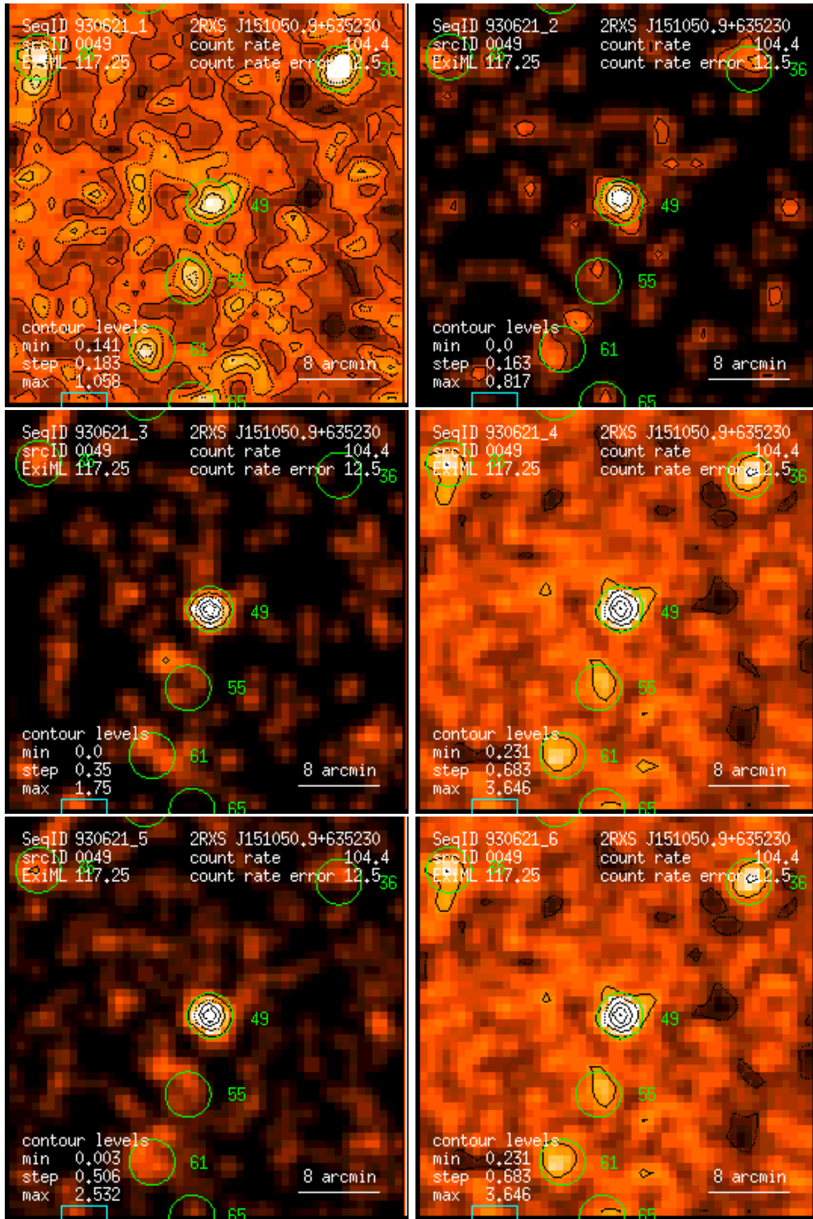
Figure 49: RASS 930621: detection 0049: band rate images, Gaussian filter: (1) PSPC channels 11 – 41, (2) 52 – 90, (3) 91 – 201, (4) 11 – 235, (5) 52 – 201, (6) 11 – 201. Broad band rates in counts/ks. Band rate contour levels in counts/ks/arcmin 2 .
