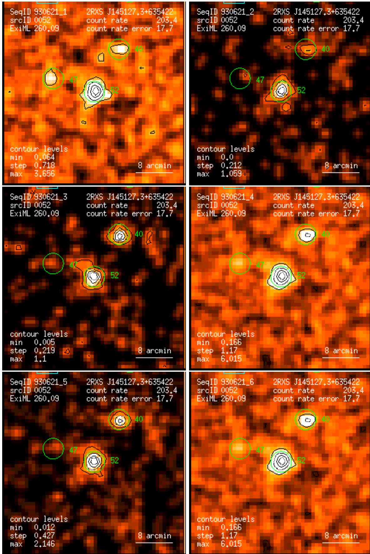
Figure 52: RASS 930621: detection 0052: band rate images, Gaussian filter: (1) PSPC channels 11 – 41, (2) 52 – 90, (3) 91 – 201, (4) 11 – 235, (5) 52 – 201, (6) 11 – 201. Broad band rates in counts/ks. Band rate contour levels in counts/ks/arcmin 2 .
