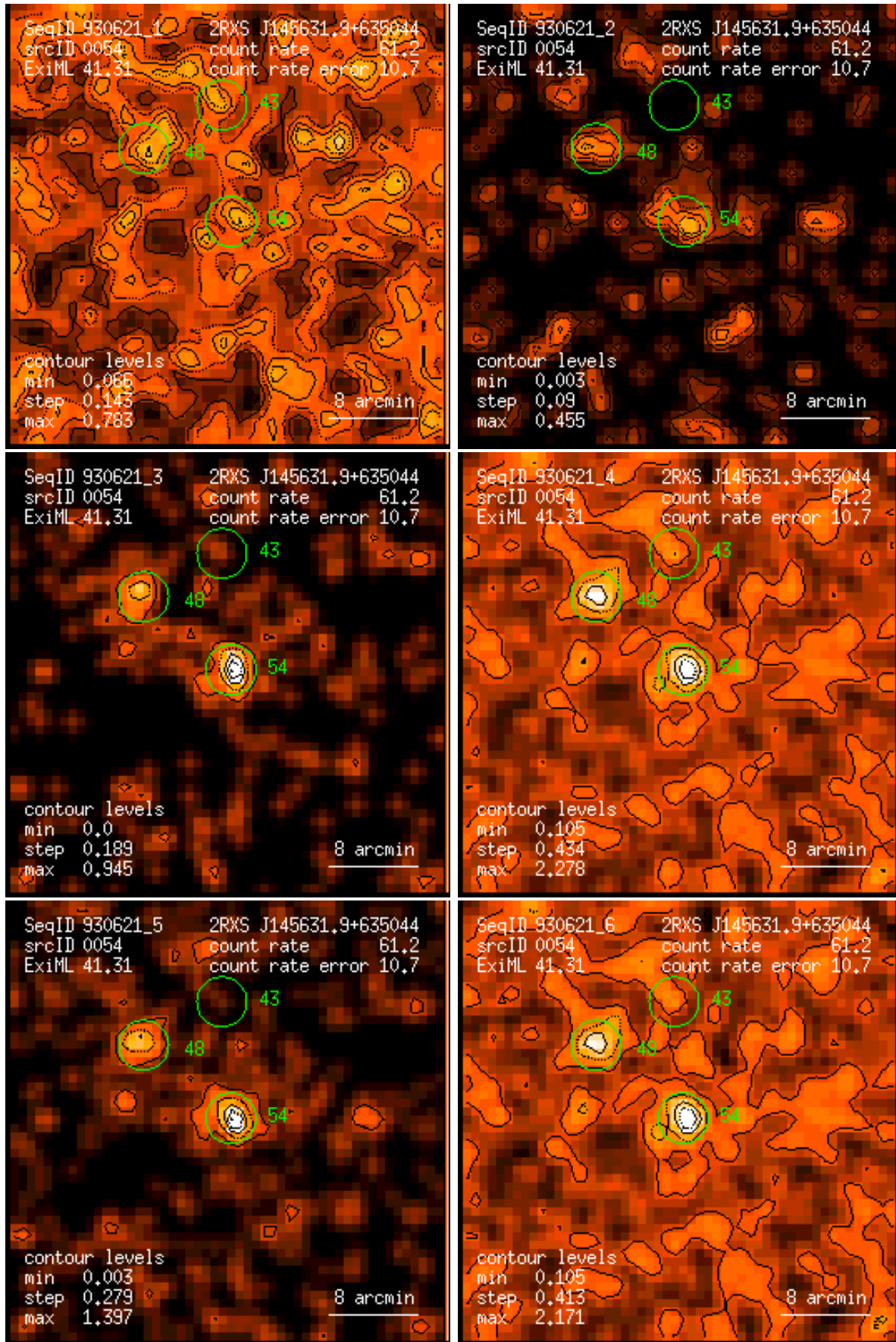
Figure 54: RASS 930621: detection 0054: band rate images, Gaussian filter: (1) PSPC channels 11 – 41, (2) 52 – 90, (3) 91 – 201, (4) 11 – 235, (5) 52 – 201, (6) 11 – 201. Broad band rates in counts/ks. Band rate contour levels in counts/ks/arcmin 2 .
