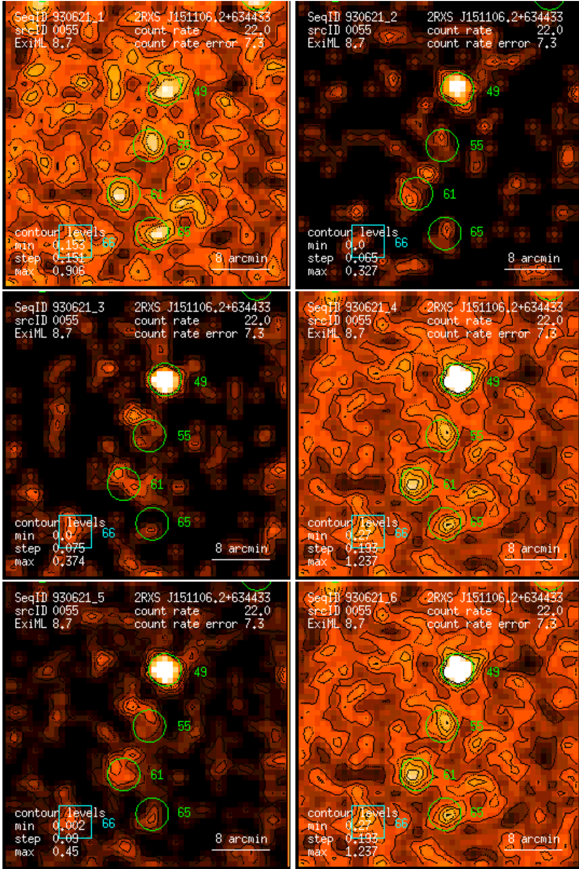
Figure 55: RASS 930621: detection 0055: band rate images, Gaussian filter: (1) PSPC channels 11 – 41, (2) 52 – 90, (3) 91 – 201, (4) 11 – 235, (5) 52 – 201, (6) 11 – 201. Broad band rates in counts/ks. Band rate contour levels in counts/ks/arcmin 2 .
