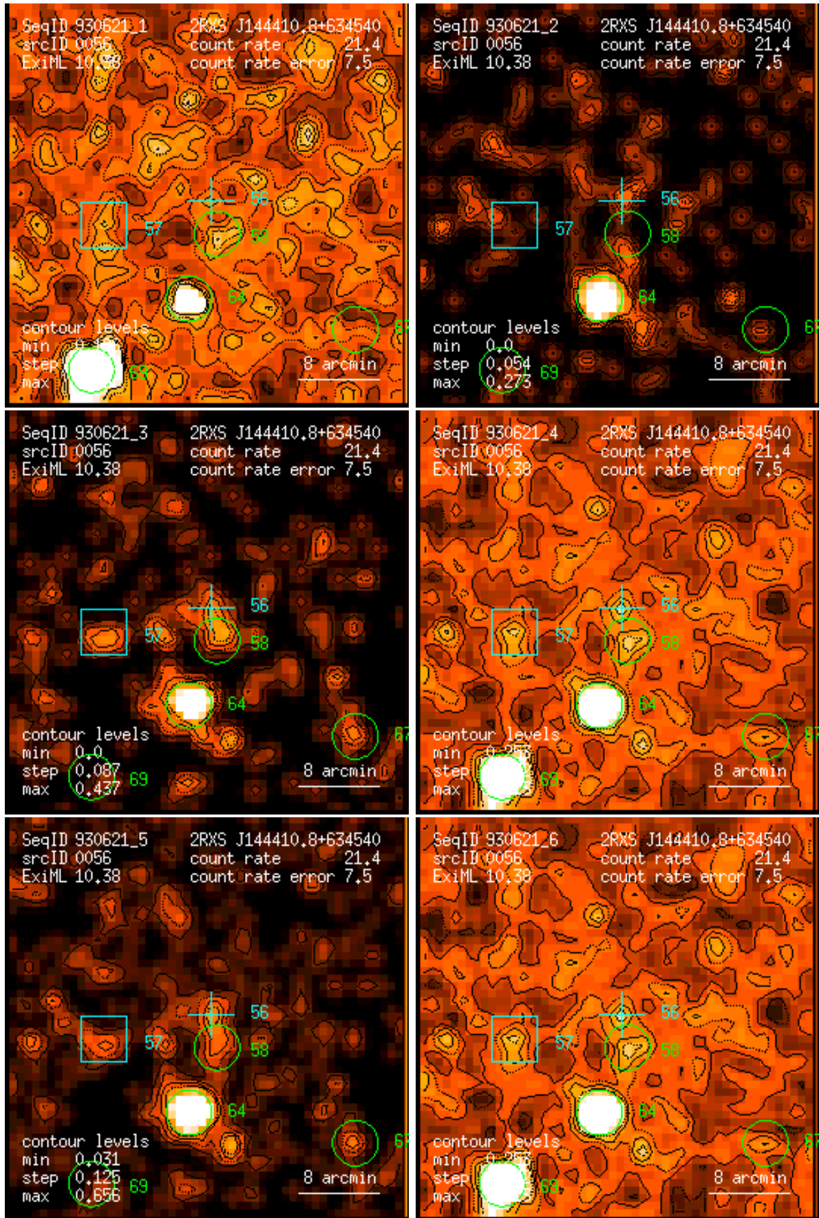
Figure 56: RASS 930621: detection 0056: band rate images, Gaussian filter: (1) PSPC channels 11 – 41, (2) 52 – 90, (3) 91 – 201, (4) 11 – 235, (5) 52 – 201, (6) 11 – 201. Broad band rates in counts/ks. Band rate contour levels in counts/ks/arcmin 2 .
