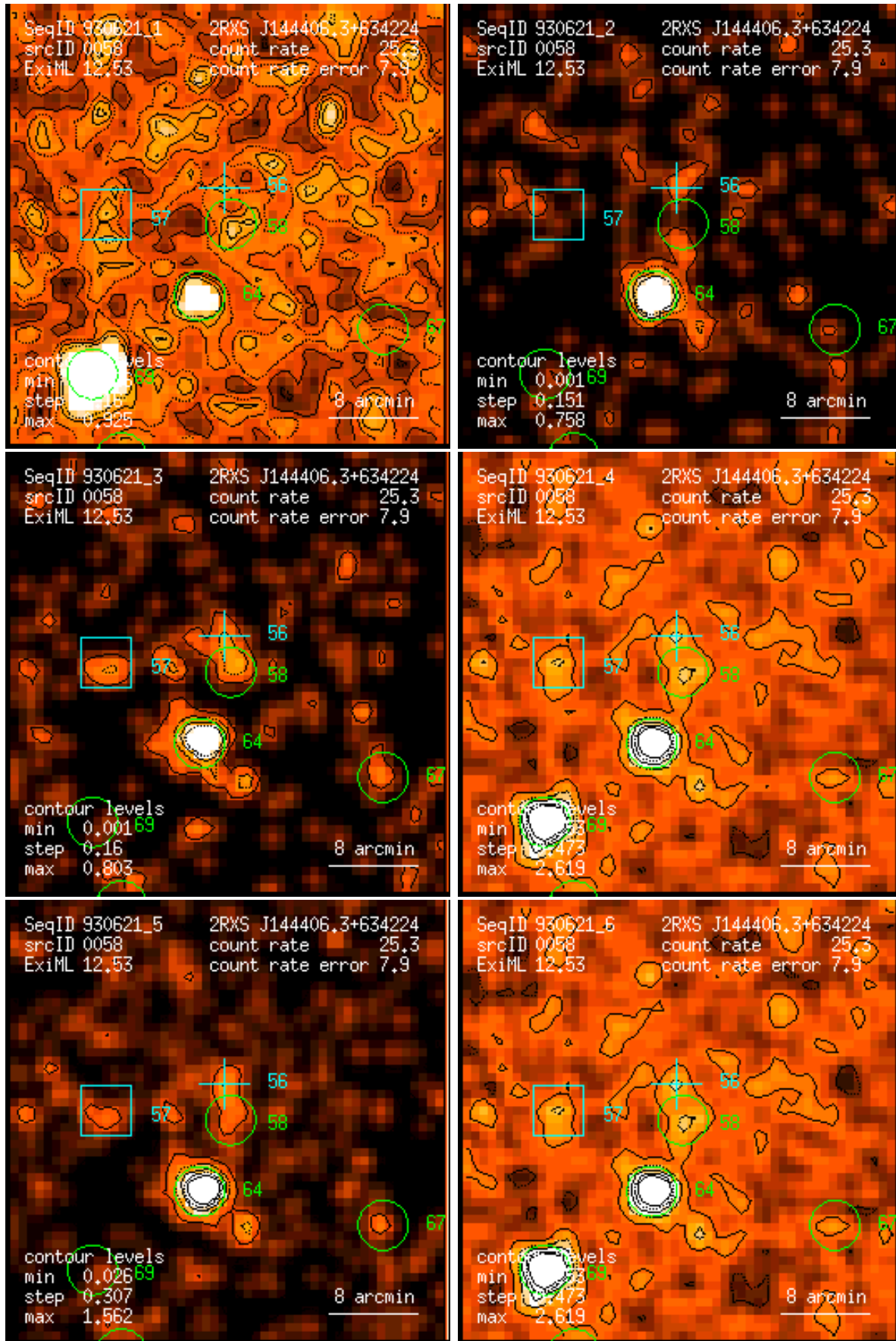
Figure 58: RASS 930621: detection 0058: band rate images, Gaussian filter: (1) PSPC channels 11 – 41, (2) 52 – 90, (3) 91 – 201, (4) 11 – 235, (5) 52 – 201, (6) 11 – 201. Broad band rates in counts/ks. Band rate contour levels in counts/ks/arcmin 2 .
