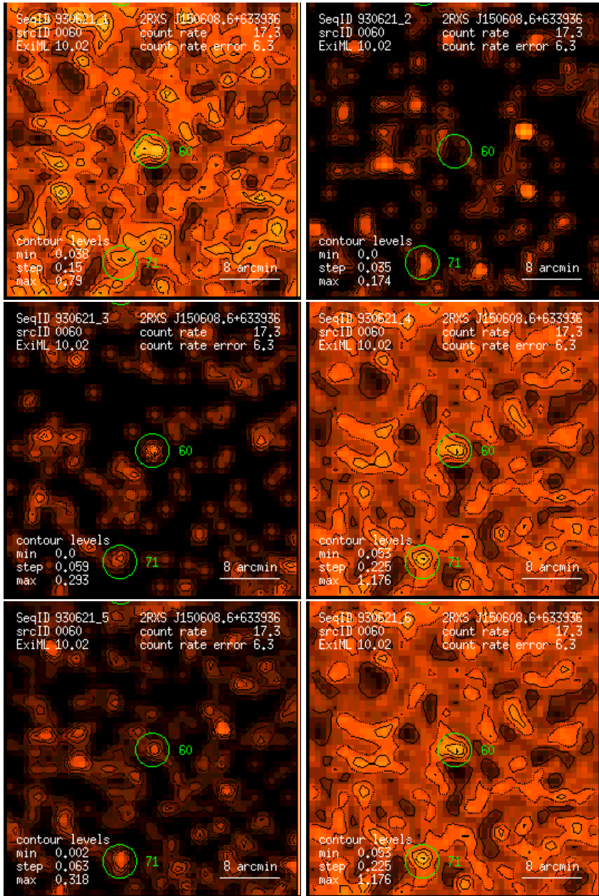
Figure 60: RASS 930621: detection 0060: band rate images, Gaussian filter: (1) PSPC channels 11 – 41, (2) 52 – 90, (3) 91 – 201, (4) 11 – 235, (5) 52 – 201, (6) 11 – 201. Broad band rates in counts/ks. Band rate contour levels in counts/ks/arcmin 2 .
