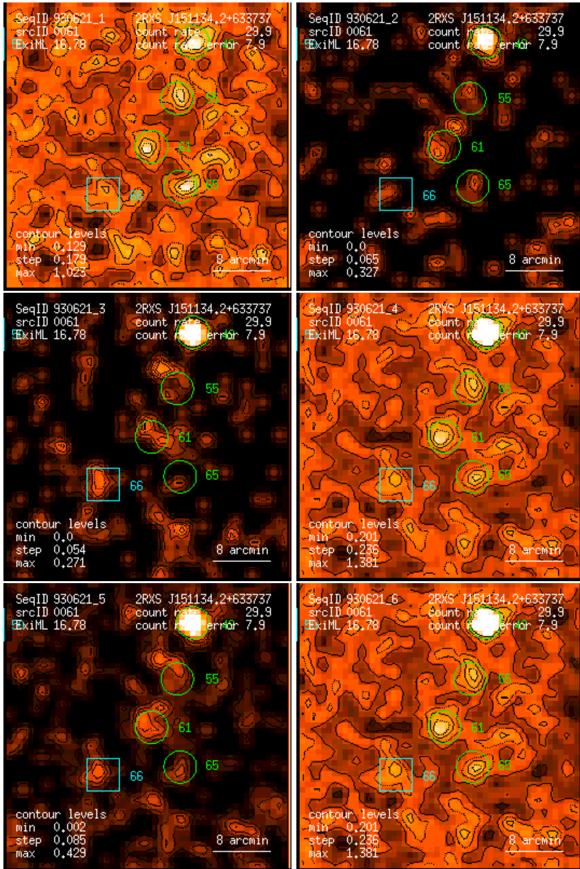
Figure 61: RASS 930621: detection 0061: band rate images, Gaussian filter: (1) PSPC channels 11 – 41, (2) 52 – 90, (3) 91 – 201, (4) 11 – 235, (5) 52 – 201, (6) 11 – 201. Broad band rates in counts/ks. Band rate contour levels in counts/ks/arcmin 2 .
