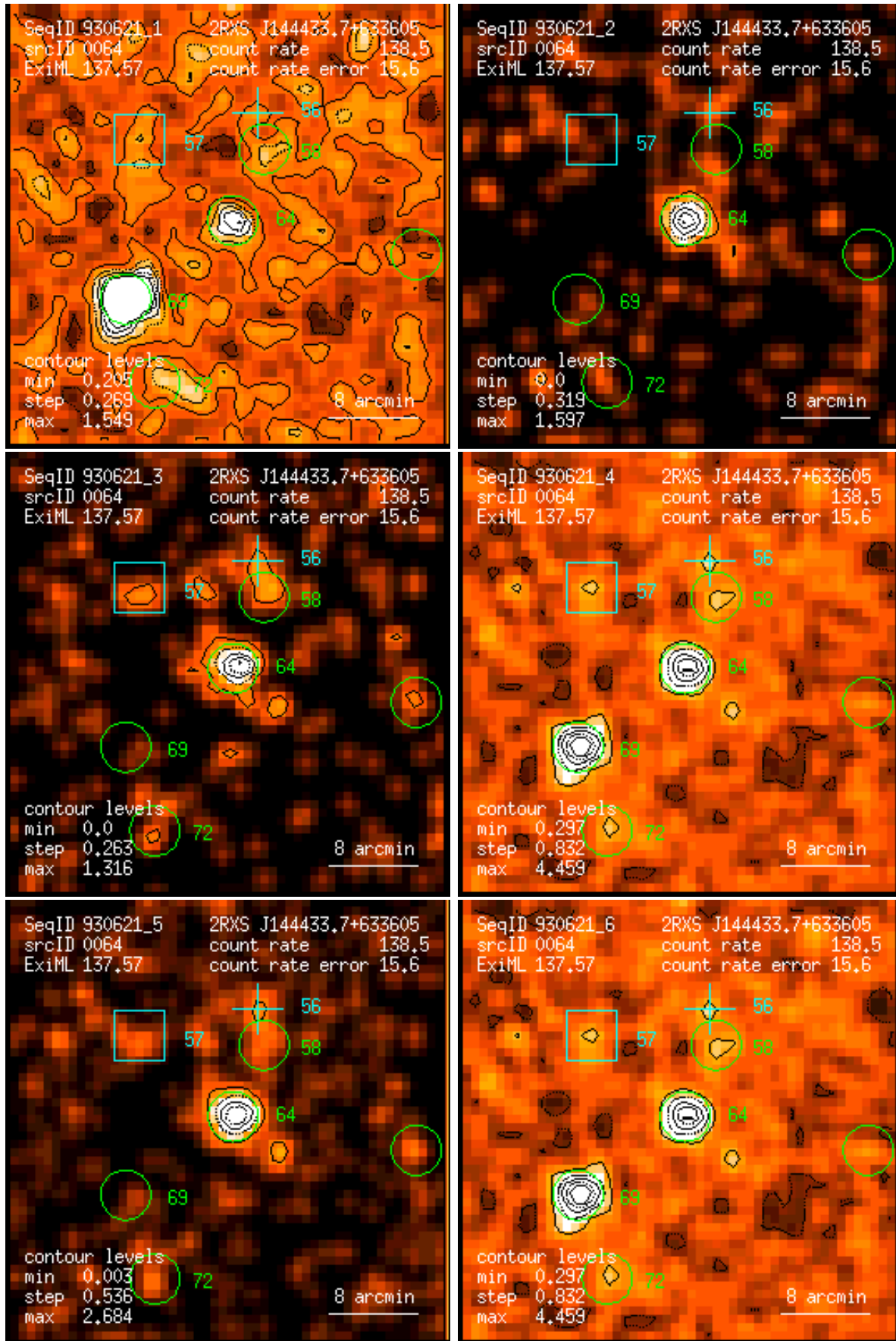
Figure 64: RASS 930621: detection 0064: band rate images, Gaussian filter: (1) PSPC channels 11 – 41, (2) 52 – 90, (3) 91 – 201, (4) 11 – 235, (5) 52 – 201, (6) 11 – 201. Broad band rates in counts/ks. Band rate contour levels in counts/ks/arcmin 2 .
