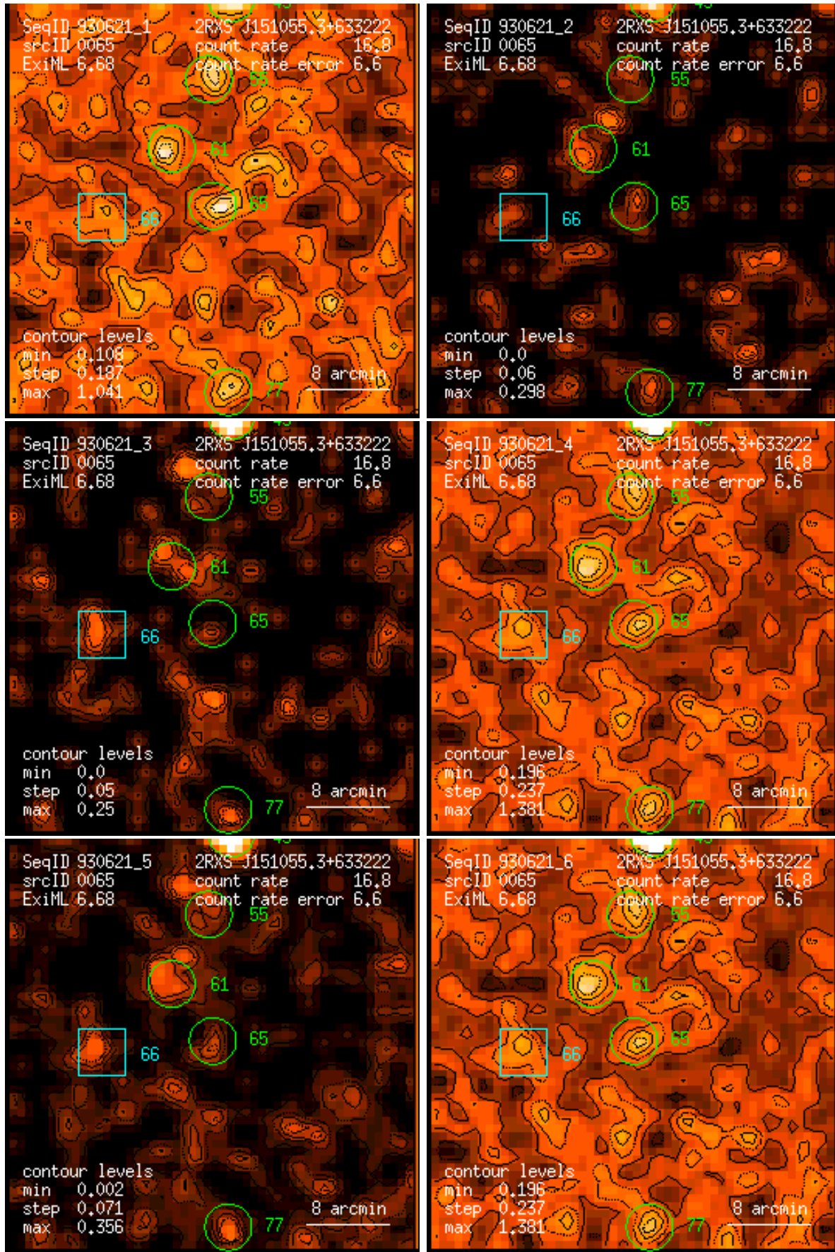
Figure 65: RASS 930621: detection 0065: band rate images, Gaussian filter: (1) PSPC channels 11 – 41, (2) 52 – 90, (3) 91 – 201, (4) 11 – 235, (5) 52 – 201, (6) 11 – 201. Broad band rates in counts/ks. Band rate contour levels in counts/ks/arcmin 2 .
