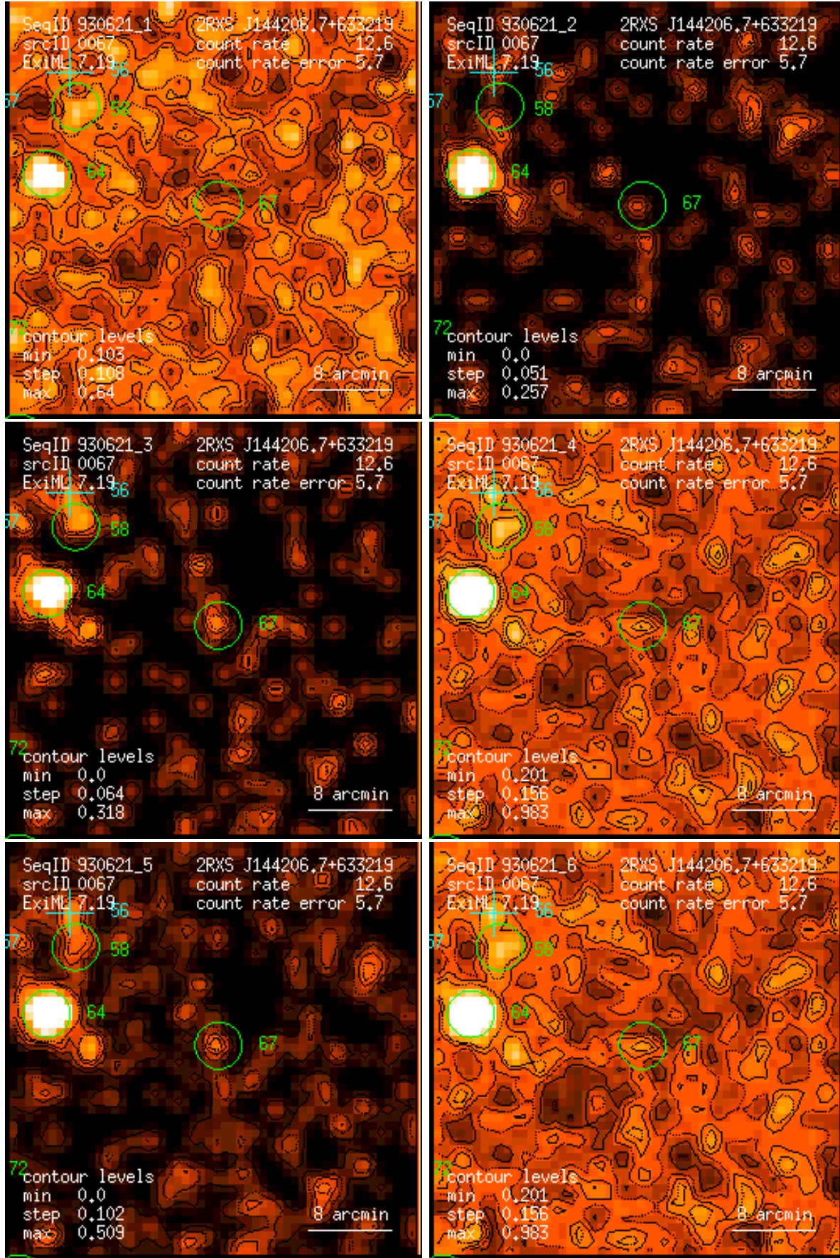
Figure 67: RASS 930621: detection 0067: band rate images, Gaussian filter: (1) PSPC channels 11 – 41, (2) 52 – 90, (3) 91 – 201, (4) 11 – 235, (5) 52 – 201, (6) 11 – 201. Broad band rates in counts/ks. Band rate contour levels in counts/ks/arcmin 2 .
