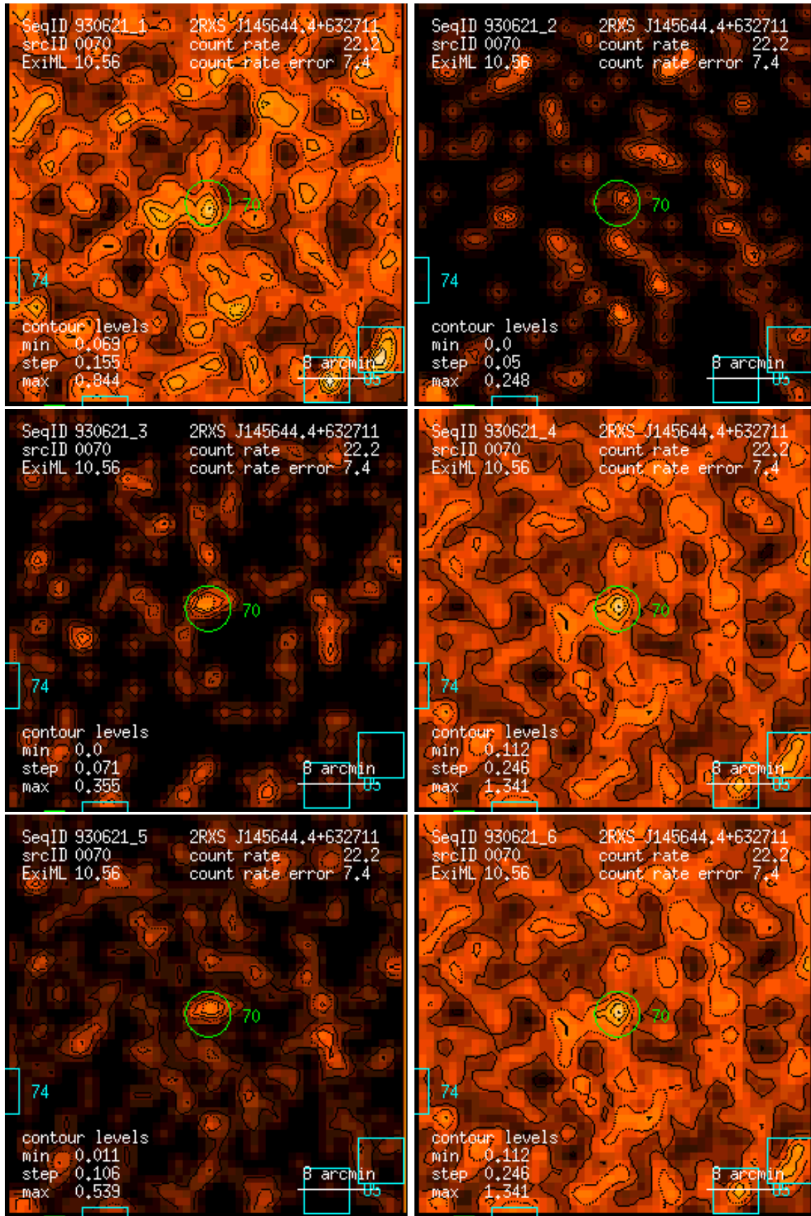
Figure 70: RASS 930621: detection 0070: band rate images, Gaussian filter: (1) PSPC channels 11 – 41, (2) 52 – 90, (3) 91 – 201, (4) 11 – 235, (5) 52 – 201, (6) 11 – 201. Broad band rates in counts/ks. Band rate contour levels in counts/ks/arcmin 2 .
