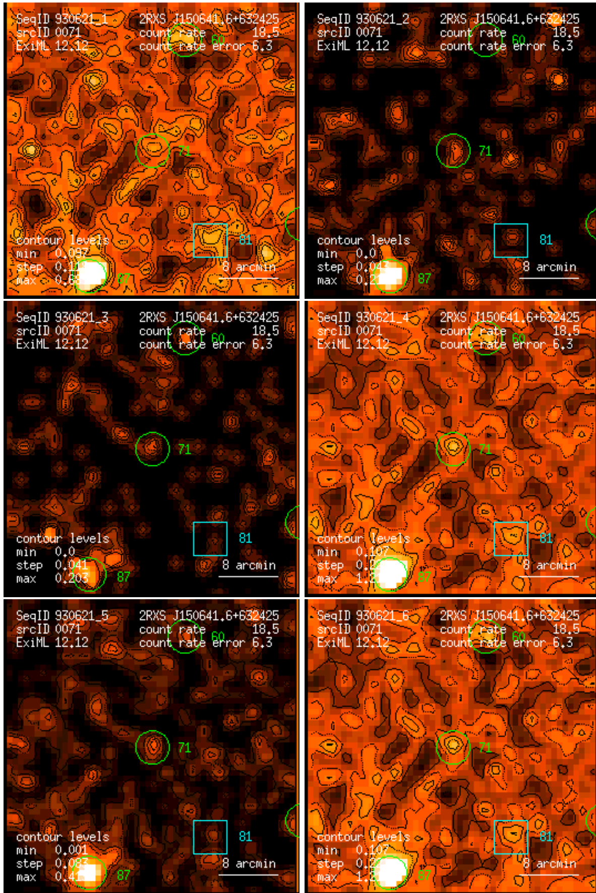
Figure 71: RASS 930621: detection 0071: band rate images, Gaussian filter: (1) PSPC channels 11 – 41, (2) 52 – 90, (3) 91 – 201, (4) 11 – 235, (5) 52 – 201, (6) 11 – 201. Broad band rates in counts/ks. Band rate contour levels in counts/ks/arcmin 2 .
