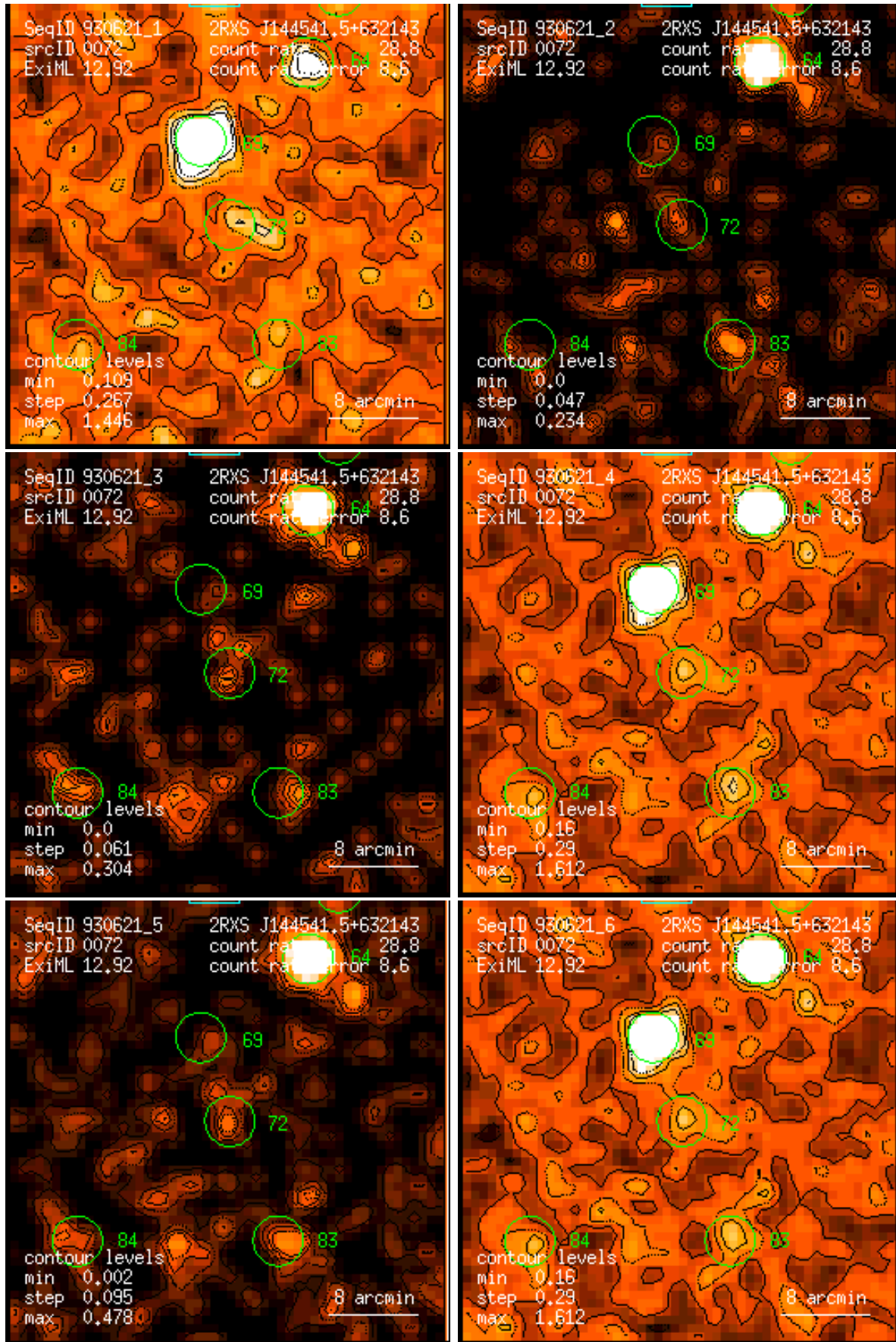
Figure 72: RASS 930621: detection 0072: band rate images, Gaussian filter: (1) PSPC channels 11 – 41, (2) 52 – 90, (3) 91 – 201, (4) 11 – 235, (5) 52 – 201, (6) 11 – 201. Broad band rates in counts/ks. Band rate contour levels in counts/ks/arcmin 2 .
