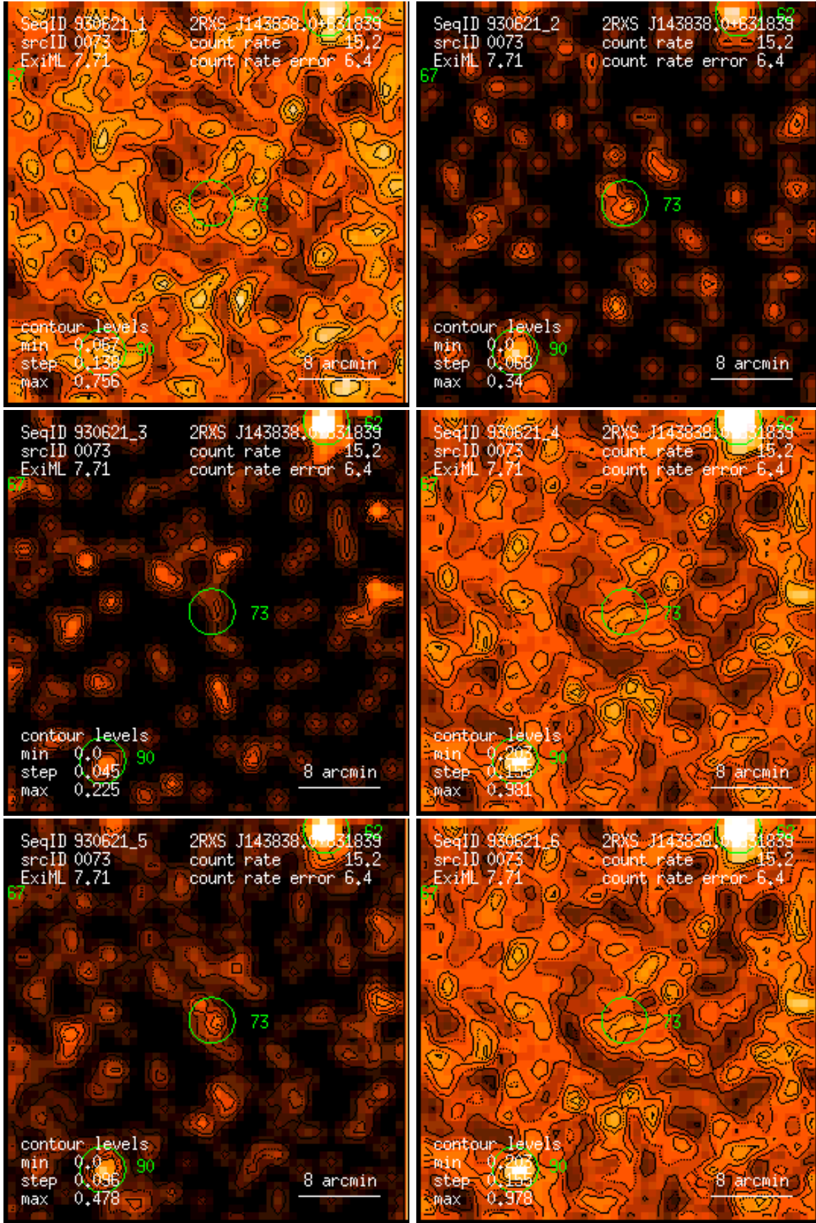
Figure 73: RASS 930621: detection 0073: band rate images, Gaussian filter: (1) PSPC channels 11 – 41, (2) 52 – 90, (3) 91 – 201, (4) 11 – 235, (5) 52 – 201, (6) 11 – 201. Broad band rates in counts/ks. Band rate contour levels in counts/ks/arcmin 2 .
