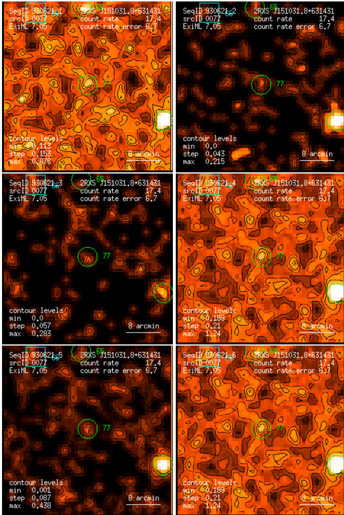
Figure 77: RASS 930621: detection 0077: band rate images, Gaussian filter: (1) PSPC channels 11 – 41, (2) 52 – 90, (3) 91 – 201, (4) 11 – 235, (5) 52 – 201, (6) 11 – 201. Broad band rates in counts/ks. Band rate contour levels in counts/ks/arcmin 2 .
