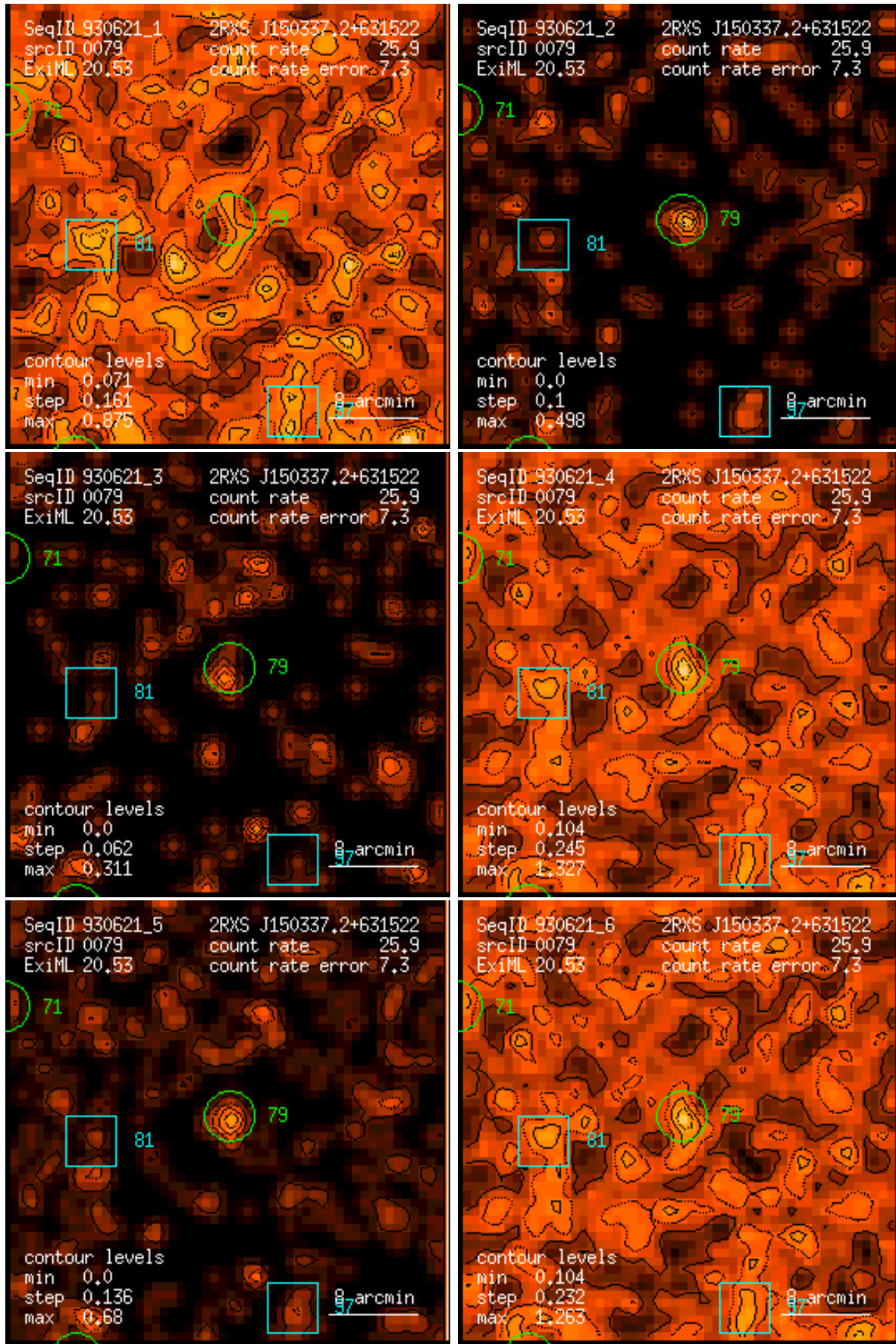
Figure 79: RASS 930621: detection 0079: band rate images, Gaussian filter: (1) PSPC channels 11 – 41, (2) 52 – 90, (3) 91 – 201, (4) 11 – 235, (5) 52 – 201, (6) 11 – 201. Broad band rates in counts/ks. Band rate contour levels in counts/ks/arcmin 2 .
