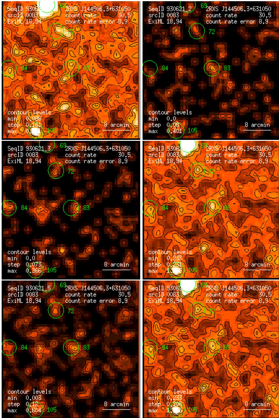
Figure 83: RASS 930621: detection 0083: band rate images, Gaussian filter: (1) PSPC channels 11 – 41, (2) 52 – 90, (3) 91 – 201, (4) 11 – 235, (5) 52 – 201, (6) 11 – 201. Broad band rates in counts/ks. Band rate contour levels in counts/ks/arcmin 2 .
