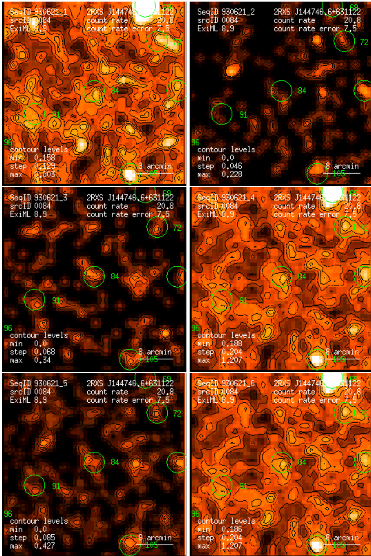
Figure 84: RASS 930621: detection 0084: band rate images, Gaussian filter: (1) PSPC channels 11 – 41, (2) 52 – 90, (3) 91 – 201, (4) 11 – 235, (5) 52 – 201, (6) 11 – 201. Broad band rates in counts/ks. Band rate contour levels in counts/ks/arcmin 2 .
