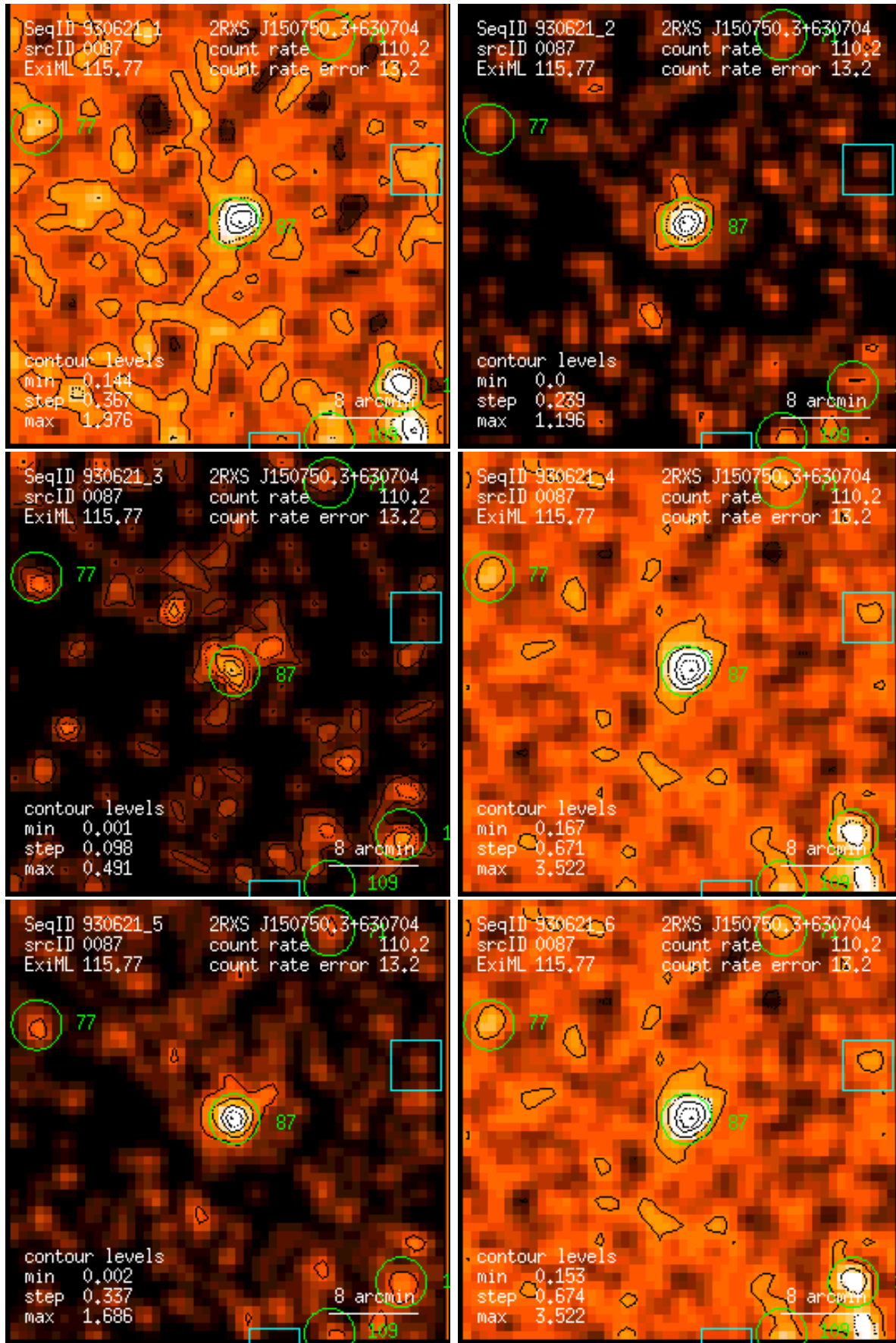
Figure 87: RASS 930621: detection 0087: band rate images, Gaussian filter: (1) PSPC channels 11 – 41, (2) 52 – 90, (3) 91 – 201, (4) 11 – 235, (5) 52 – 201, (6) 11 – 201. Broad band rates in counts/ks. Band rate contour levels in counts/ks/arcmin 2 .
