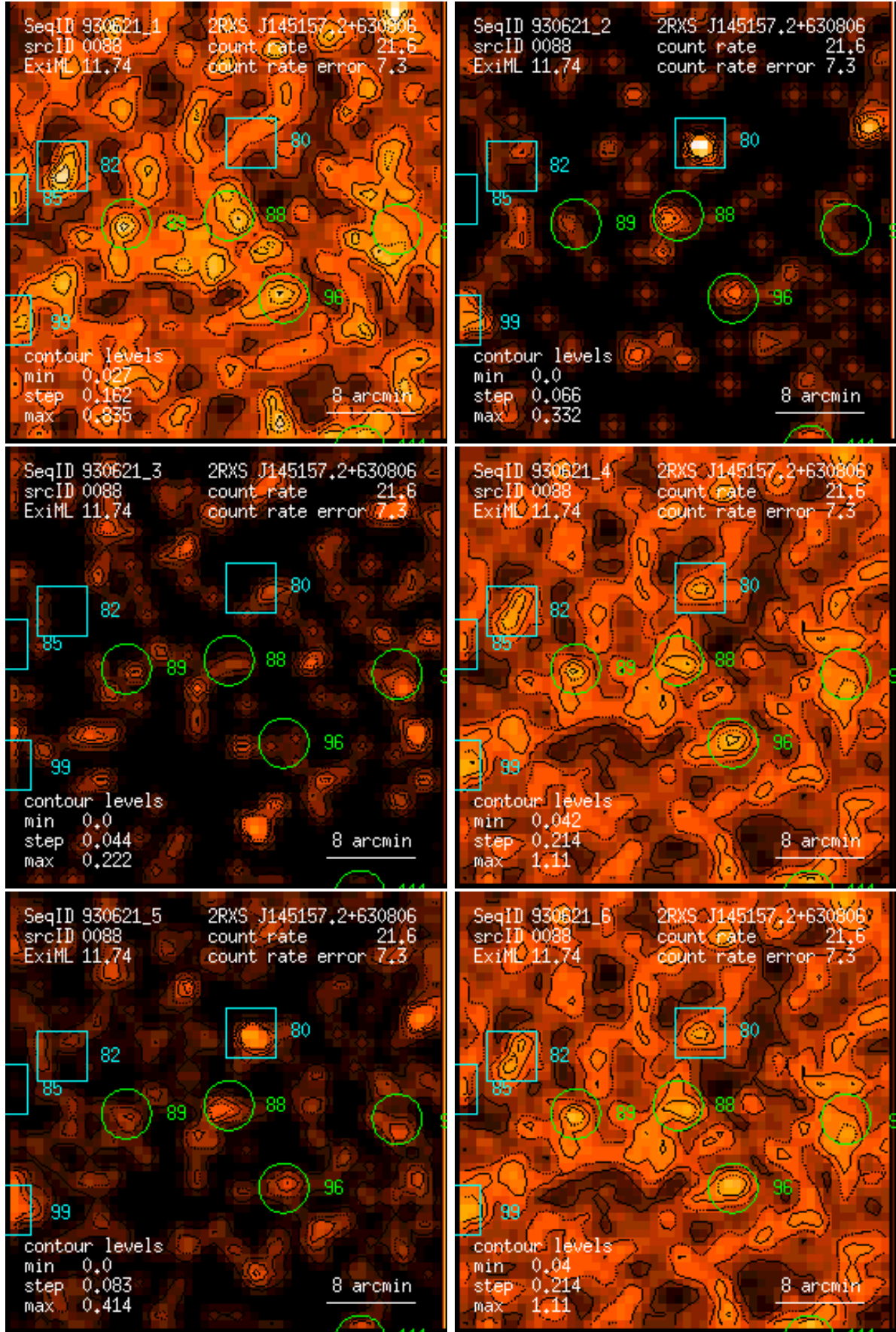
Figure 88: RASS 930621: detection 0088: band rate images, Gaussian filter: (1) PSPC channels 11 – 41, (2) 52 – 90, (3) 91 – 201, (4) 11 – 235, (5) 52 – 201, (6) 11 – 201. Broad band rates in counts/ks. Band rate contour levels in counts/ks/arcmin 2 .
