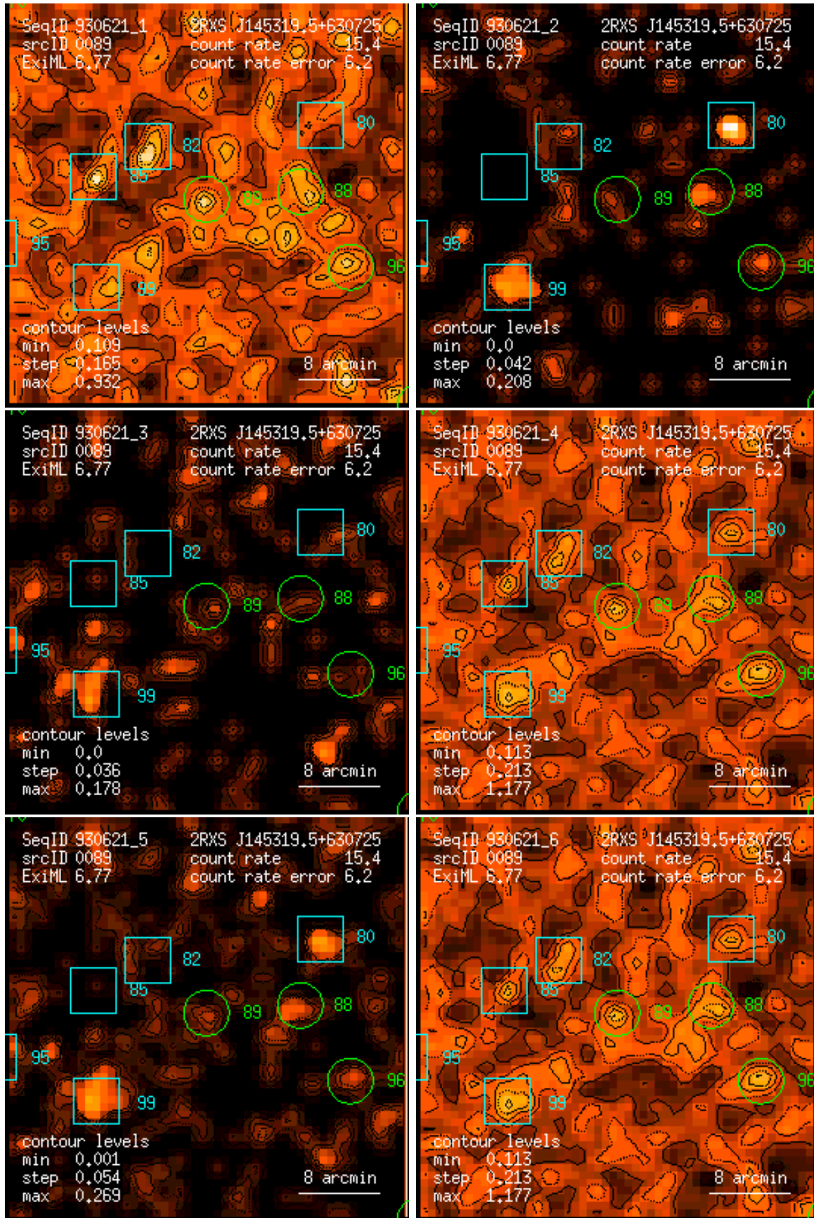
Figure 89: RASS 930621: detection 0089: band rate images, Gaussian filter: (1) PSPC channels 11 – 41, (2) 52 – 90, (3) 91 – 201, (4) 11 – 235, (5) 52 – 201, (6) 11 – 201. Broad band rates in counts/ks. Band rate contour levels in counts/ks/arcmin 2 .
