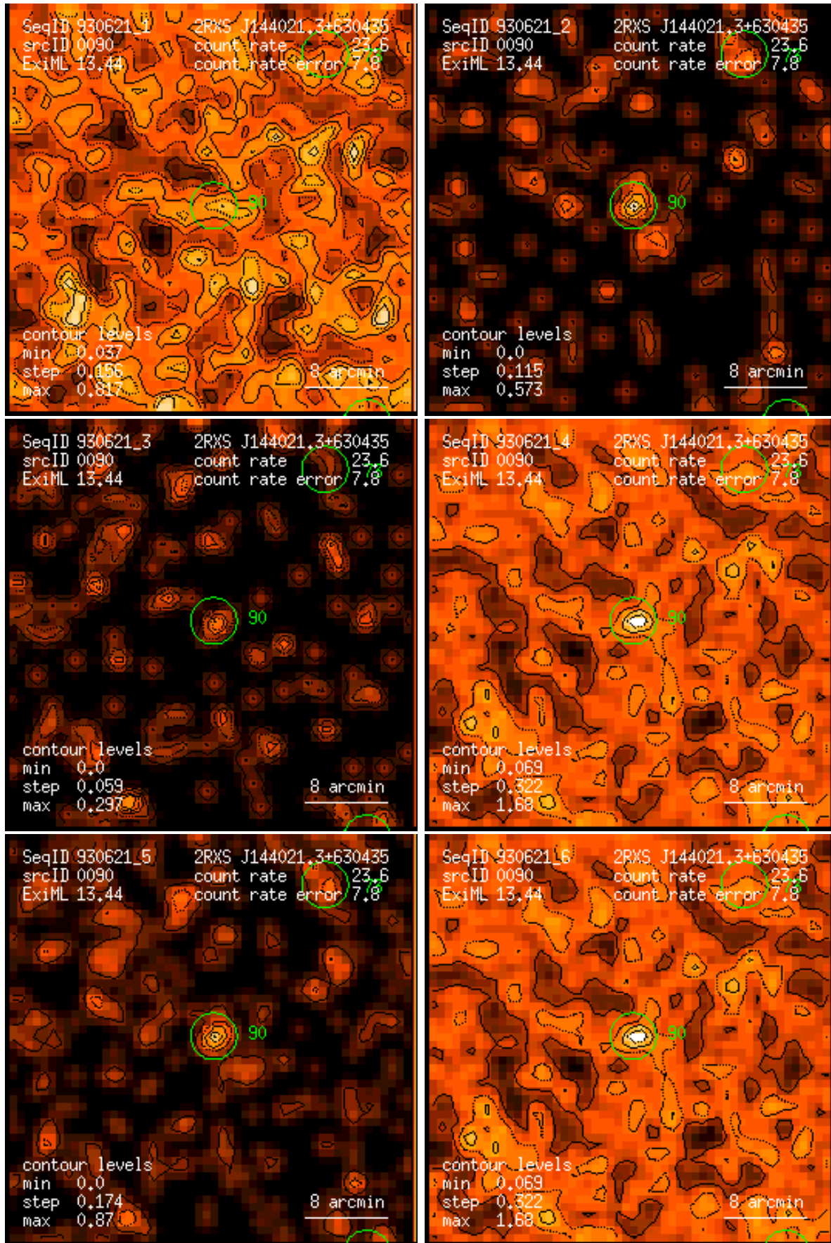
Figure 90: RASS 930621: detection 0090: band rate images, Gaussian filter: (1) PSPC channels 11 – 41, (2) 52 – 90, (3) 91 – 201, (4) 11 – 235, (5) 52 – 201, (6) 11 – 201. Broad band rates in counts/ks. Band rate contour levels in counts/ks/arcmin 2 .
