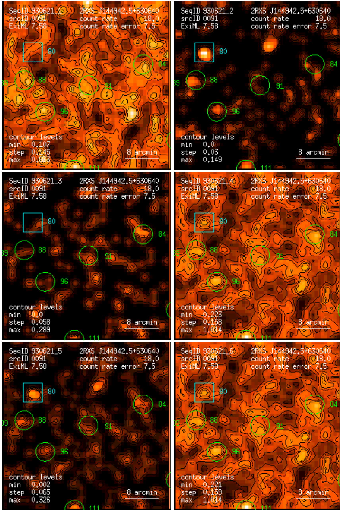
Figure 91: RASS 930621: detection 0091: band rate images, Gaussian filter: (1) PSPC channels 11 – 41, (2) 52 – 90, (3) 91 – 201, (4) 11 – 235, (5) 52 – 201, (6) 11 – 201. Broad band rates in counts/ks. Band rate contour levels in counts/ks/arcmin 2 .
