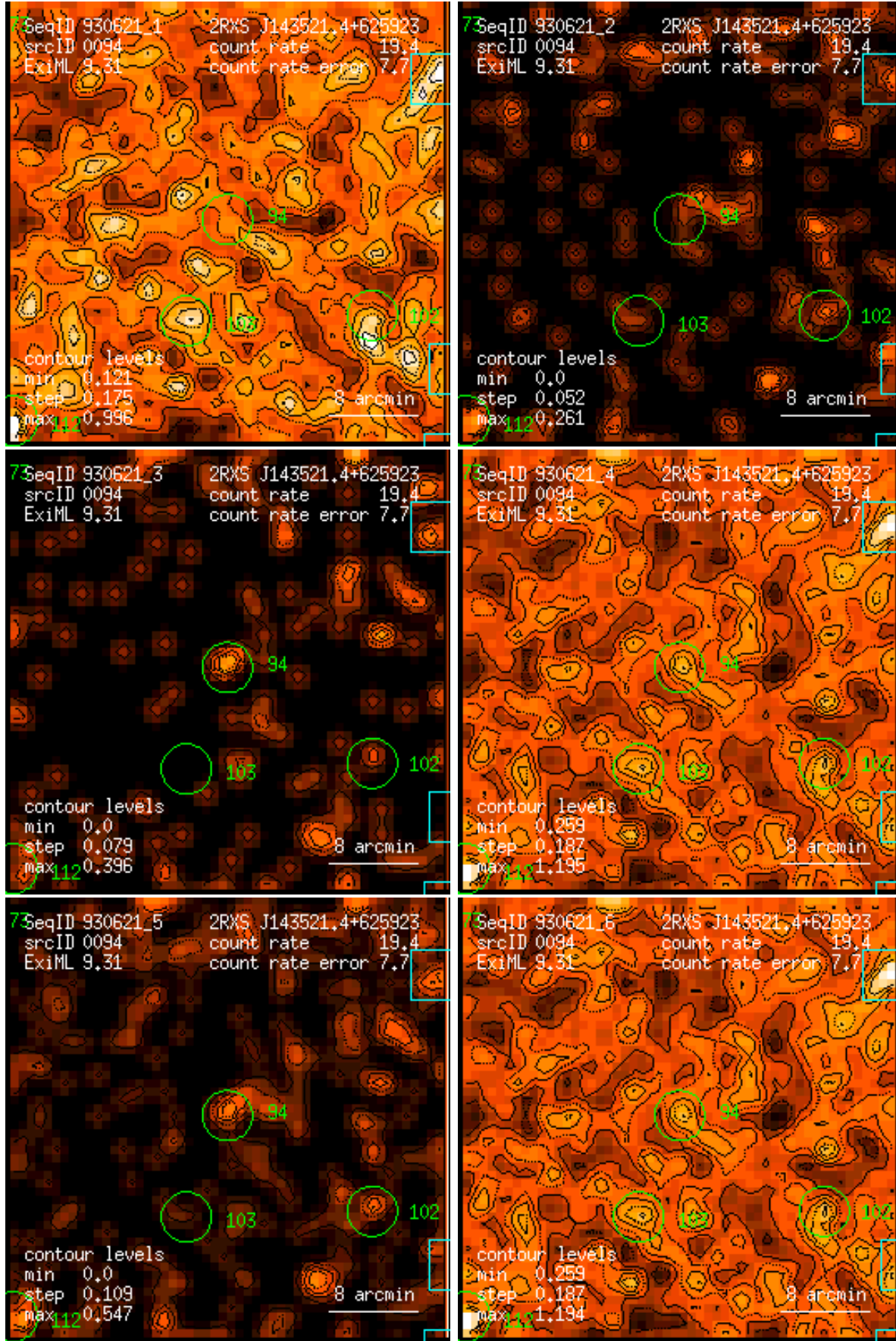
Figure 94: RASS 930621: detection 0094: band rate images, Gaussian filter: (1) PSPC channels 11 – 41, (2) 52 – 90, (3) 91 – 201, (4) 11 – 235, (5) 52 – 201, (6) 11 – 201. Broad band rates in counts/ks. Band rate contour levels in counts/ks/arcmin 2 .
