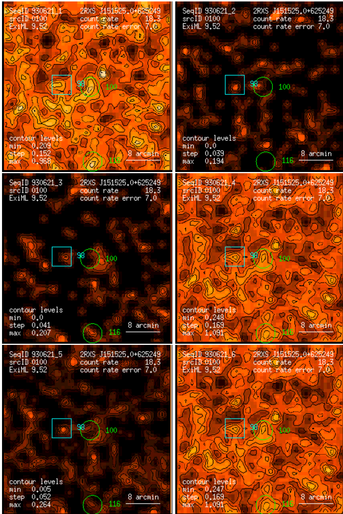
Figure 100: RASS 930621: detection 0100: band rate images, Gaussian filter: (1) PSPC channels 11 – 41, (2) 52 – 90, (3) 91 – 201, (4) 11 – 235, (5) 52 – 201, (6) 11 – 201. Broad band rates in counts/ks. Band rate contour levels in counts/ks/arcmin 2 .
