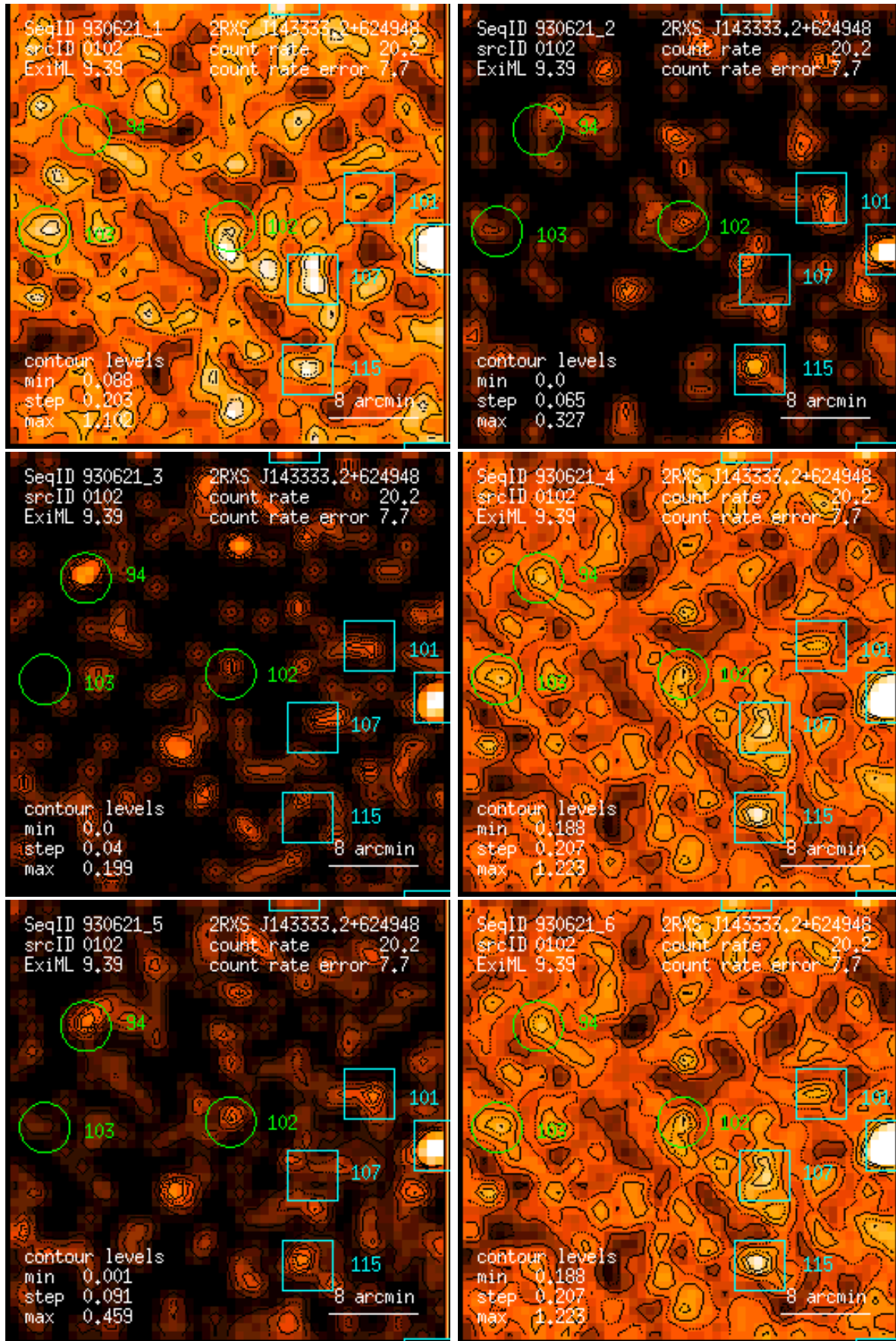
Figure 102: RASS 930621: detection 0102: band rate images, Gaussian filter: (1) PSPC channels 11 – 41, (2) 52 – 90, (3) 91 – 201, (4) 11 – 235, (5) 52 – 201, (6) 11 – 201. Broad band rates in counts/ks. Band rate contour levels in counts/ks/arcmin 2 .
