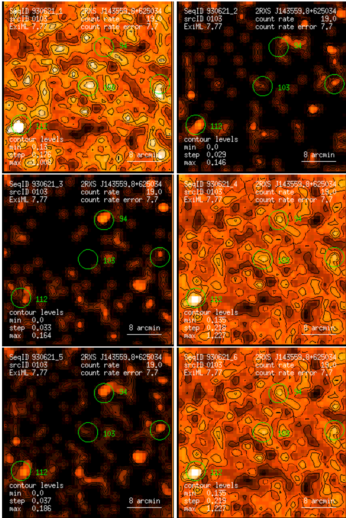
Figure 103: RASS 930621: detection 0103: band rate images, Gaussian filter: (1) PSPC channels 11 – 41, (2) 52 – 90, (3) 91 – 201, (4) 11 – 235, (5) 52 – 201, (6) 11 – 201. Broad band rates in counts/ks. Band rate contour levels in counts/ks/arcmin 2 .
