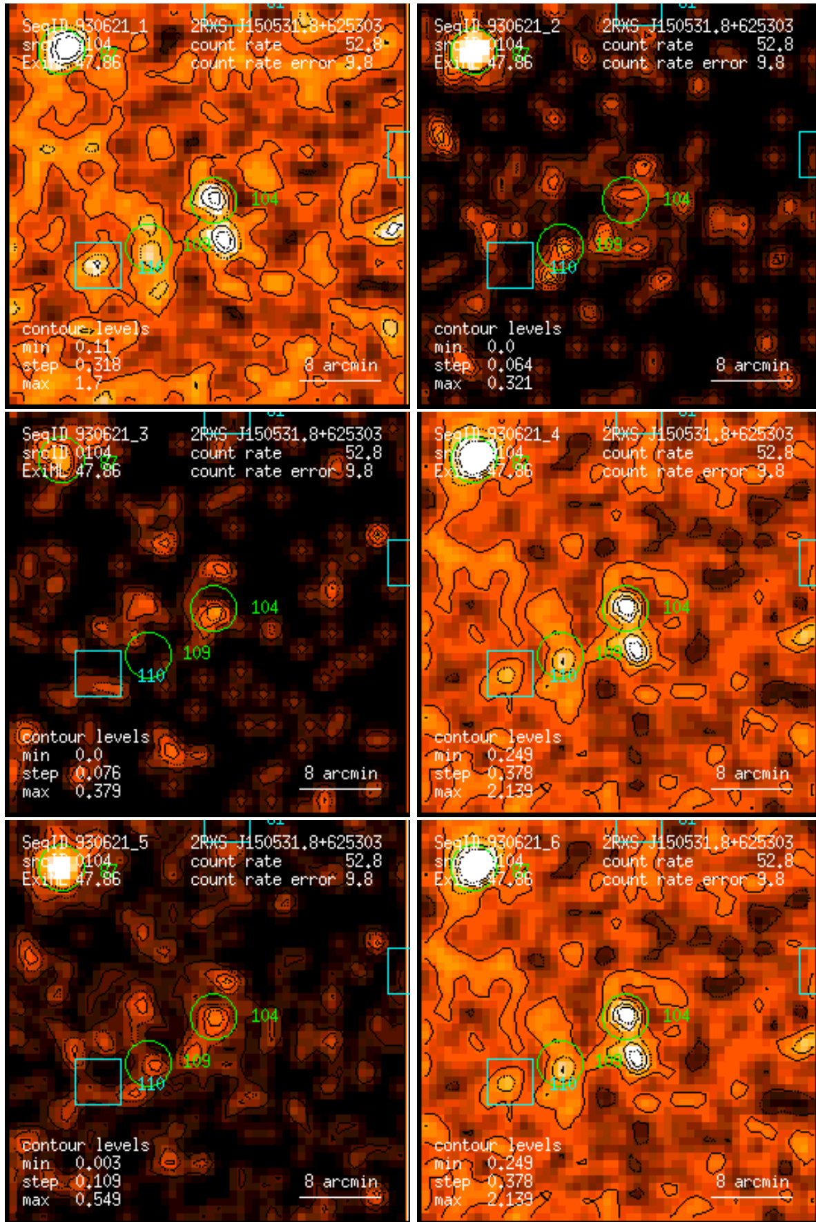
Figure 104: RASS 930621: detection 0104: band rate images, Gaussian filter: (1) PSPC channels 11 – 41, (2) 52 – 90, (3) 91 – 201, (4) 11 – 235, (5) 52 – 201, (6) 11 – 201. Broad band rates in counts/ks. Band rate contour levels in counts/ks/arcmin 2 .
