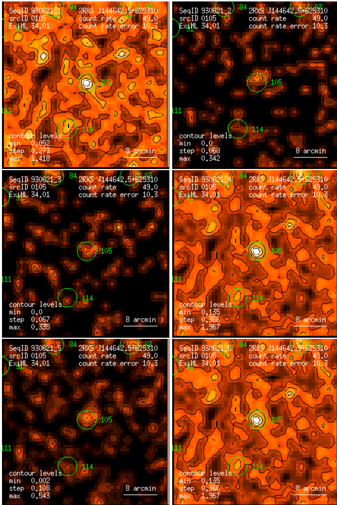
Figure 105: RASS 930621: detection 0105: band rate images, Gaussian filter: (1) PSPC channels 11 – 41, (2) 52 – 90, (3) 91 – 201, (4) 11 – 235, (5) 52 – 201, (6) 11 – 201. Broad band rates in counts/ks. Band rate contour levels in counts/ks/arcmin 2 .
